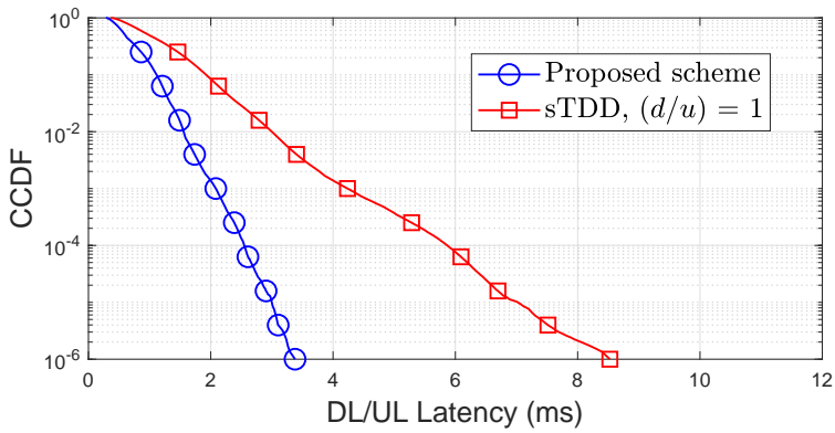
(b) UL-heavy ( \Omega^{\text{dl}} : \Omega^{\text{ul}} = 1 : 3 )
