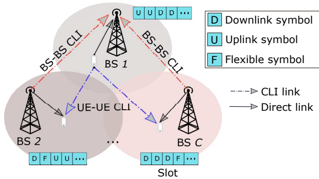
Fig. III.2: BS-BS and UE-UE CLI in dynamic TDD systems [10, Paper K].
