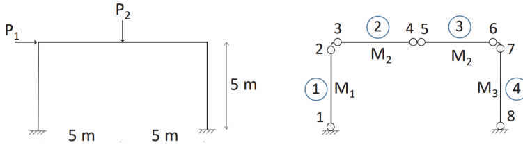
Figure E.3: Left: Portal frame structure of Example I. Right: Structural model properties.
