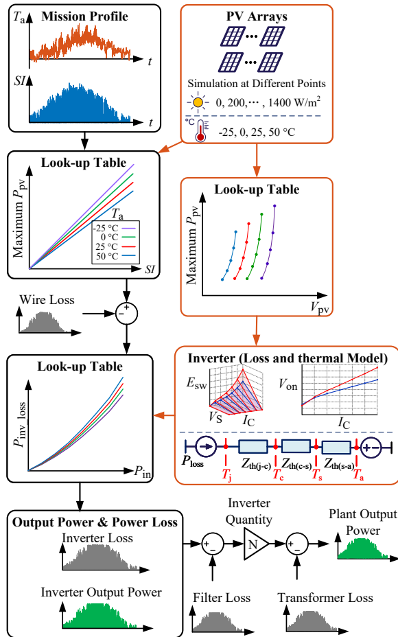
Fig. 3.3: Block diagram of the procedure for analyzing the power losses, where black and red boxes represent the main steps and the subsidiary steps, respectively. Source: [C5].
