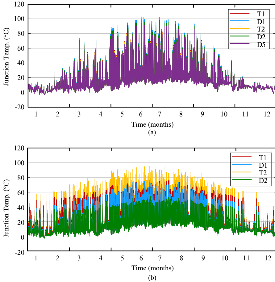
Fig. 3.13: One-year junction temperature profiles of the individual devices (referring to Fig. 3.11) in: (a) battery inverter for AC-coupling and (b) battery converter for DC-coupling. Source: [J2].
