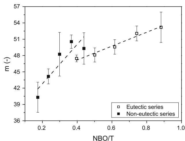
Fig. 6. The fragility or steepness index ( m ) obtained from the fragility plot versus \text{NBO}/T . The dashed lines should be regarded as guides for the eyes. The error bars represent the standard deviation of m derived from the standard deviation of F obtained from the non-linear regression of the AM equation.
