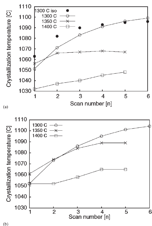
Figure 5. The change of the crystallisation peak position as a function of scan number for each maximum temperature ( T_{\text{max}} ), which is indicated in the figure labels; (a) fibre 1 and (b) fibre 2. In (a) is also included peak positions for the isothermal experiment, where the sample was kept at T_{\text{max}} (1300°C) for 15 min
