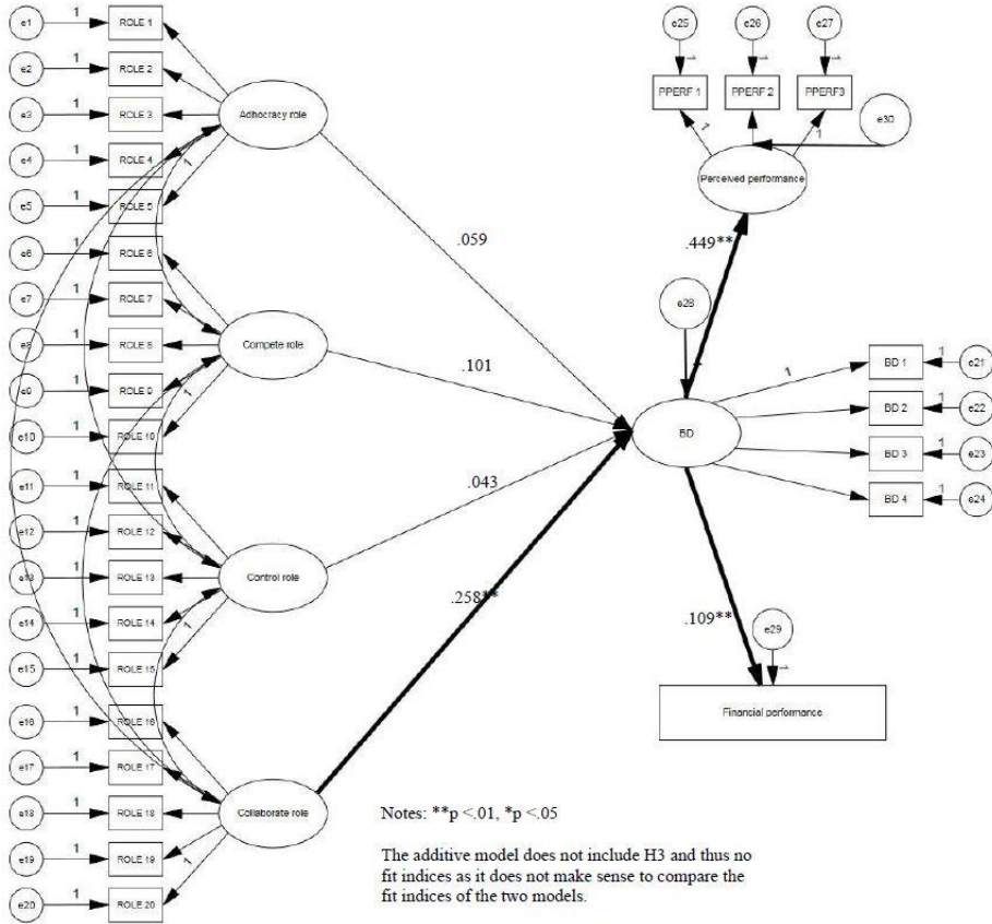
Figure 5: Additive model
