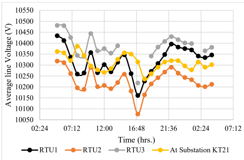
Figure 5-12 Voltage profile observed on June 1
