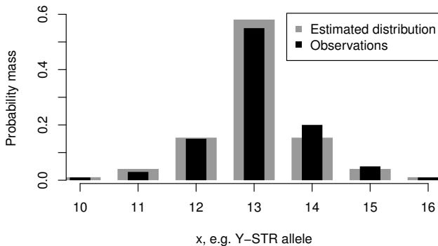
Figure 2. Observed frequencies of the x 's compared to a discrete Laplace distribution with parameters estimated from the sample.
