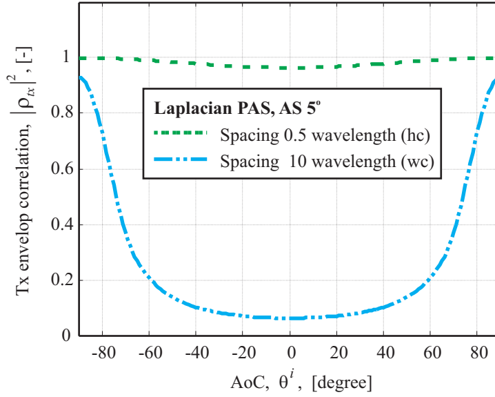
Figure 4.2: Tx envelop correlation as a function of AoC.
