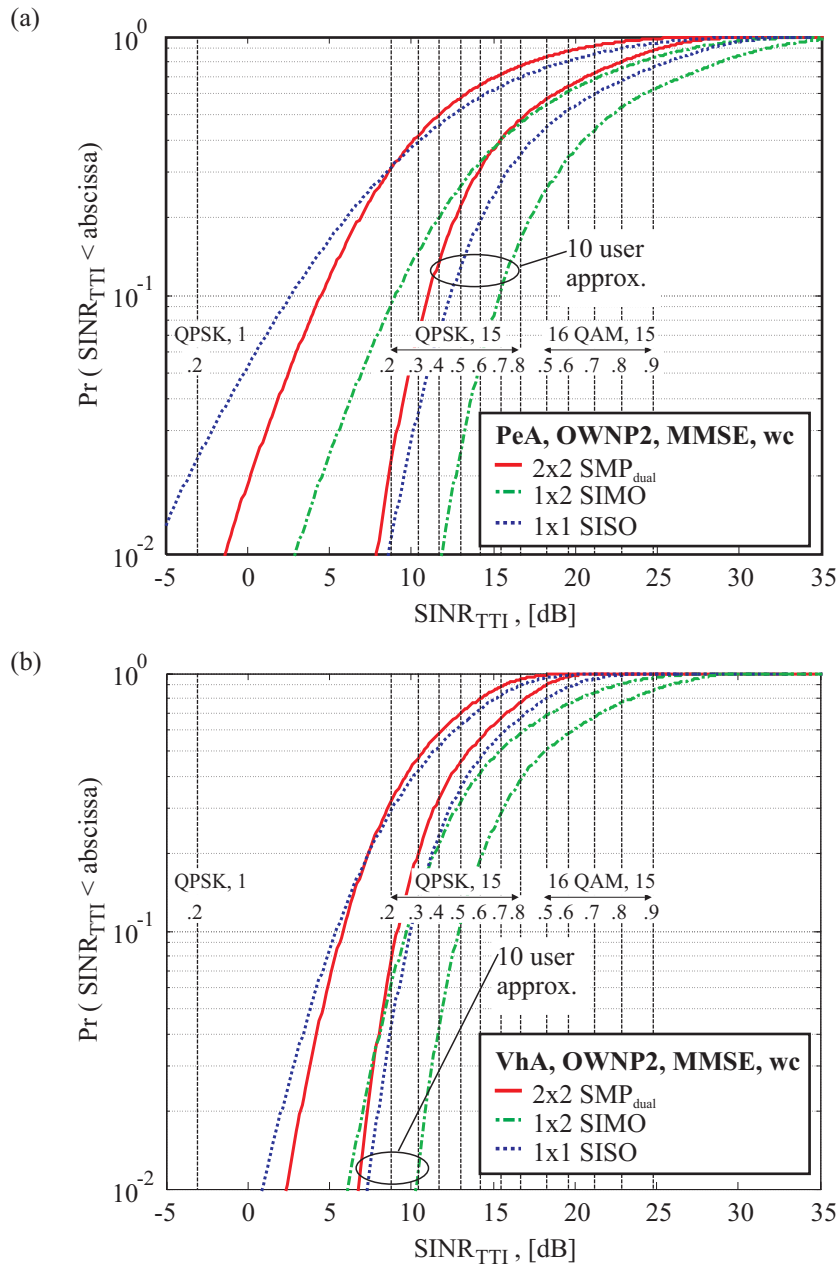
Figure 5.18: 2 \times 2 SMP_{dual} SINR statistics as encountered over the whole sector area in (a) PeA and (b) VhA. 1 \times 1 SISO and 1 \times 2 SIMO serve as references.
