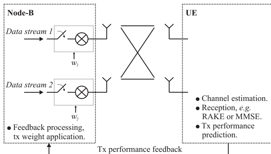
Figure 2.8: Basic SMP_x operation.
