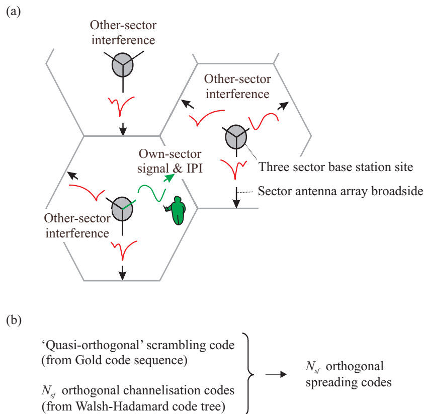
Figure 1.3: (a) Multiple access interference situation. (b) Spreading code construction.
