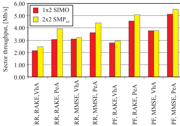
Figure 5.17: Sector throughput comparison between 1 \times 2 SIMO and 2 \times 2 SMP_{sel} for the OWNP2 model.
