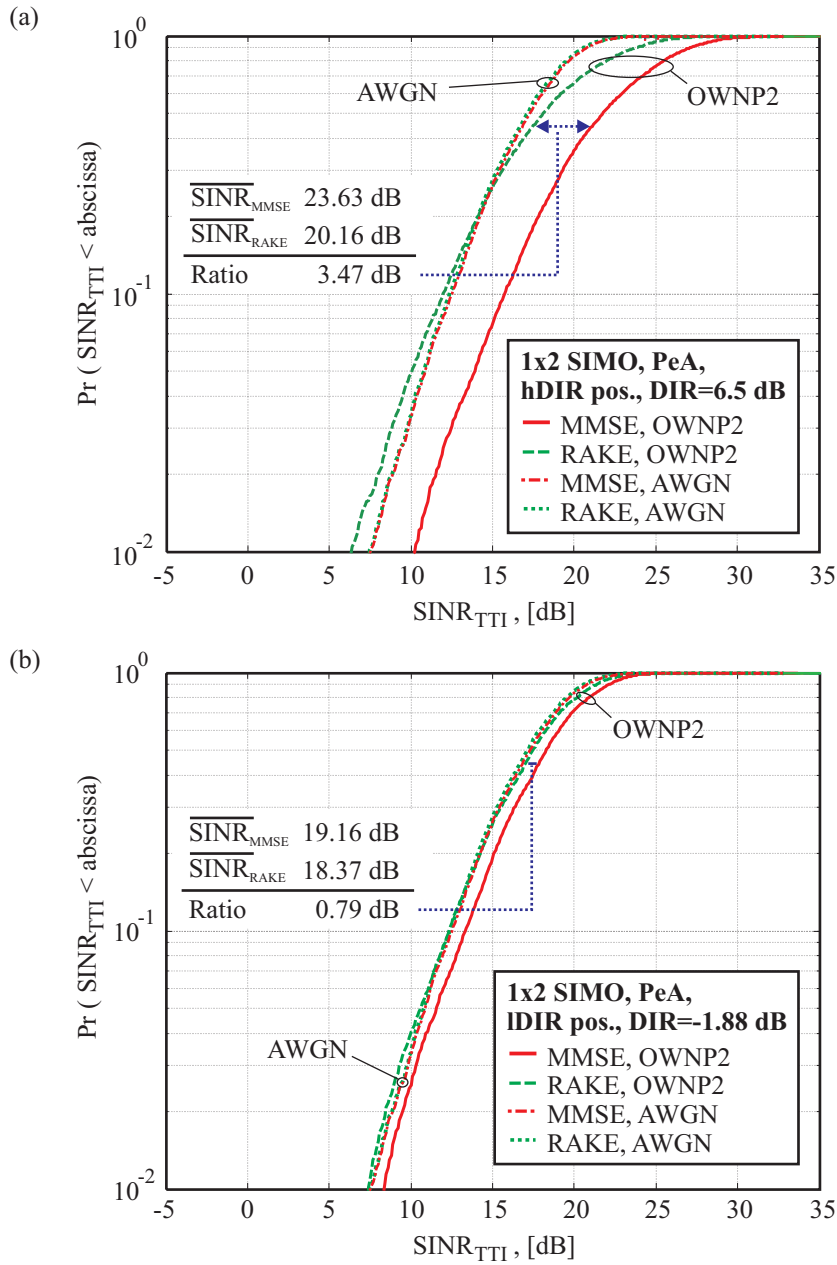
Figure 5.6: SINR cdfs of 1 \times 2 SIMO RAKE and MMSE receiver to reveal the spatial interference suppression benefit of the MMSE. (a) hDIR position. (b) IDIR position.
