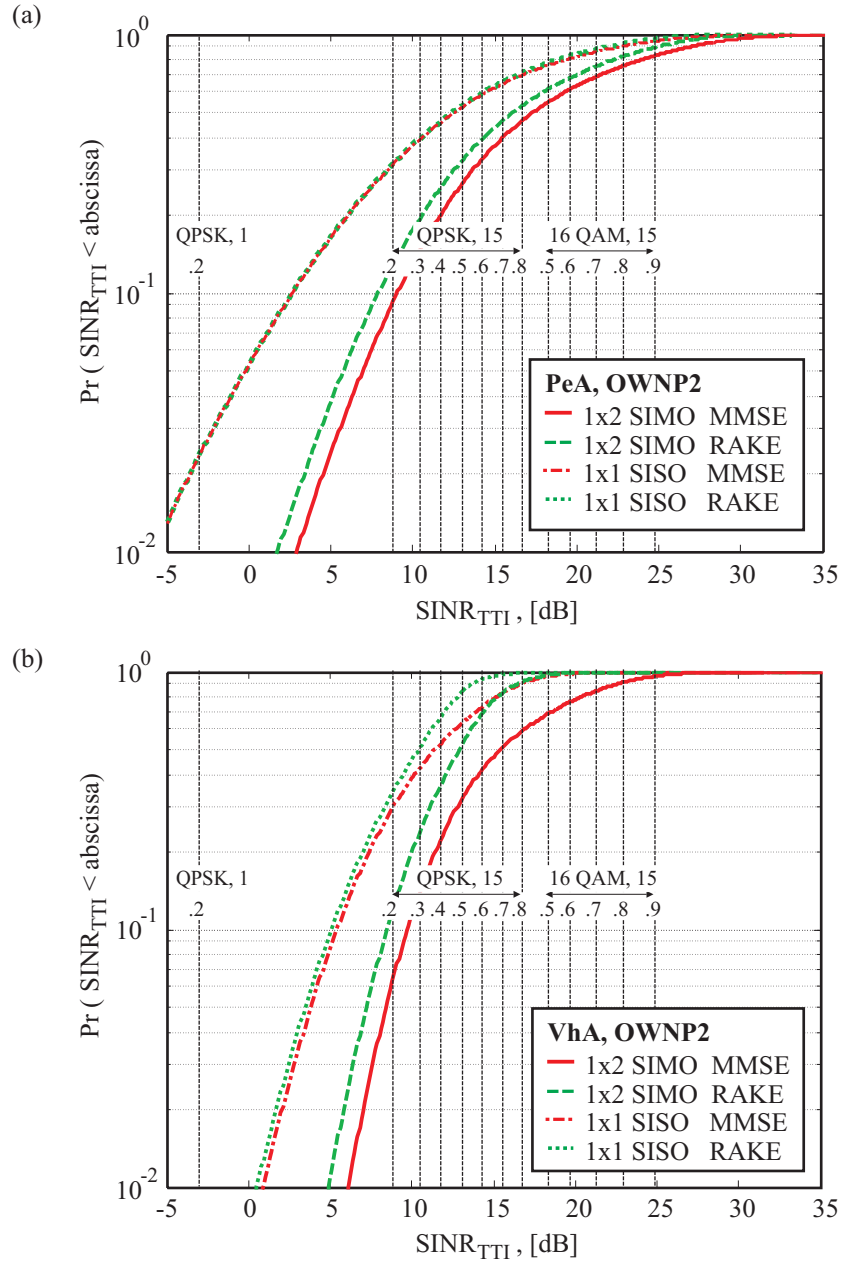
Figure 5.9: SINR statistics of 1 \times 1 SISO and 1 \times 2 SIMO scheme under the OWNP2 interference model as seen over the whole sector area.
