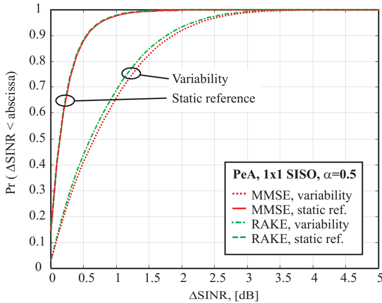
Figure 5.4: Comparison of \Delta SINR cdfs for the variability and the static reference set-up.
