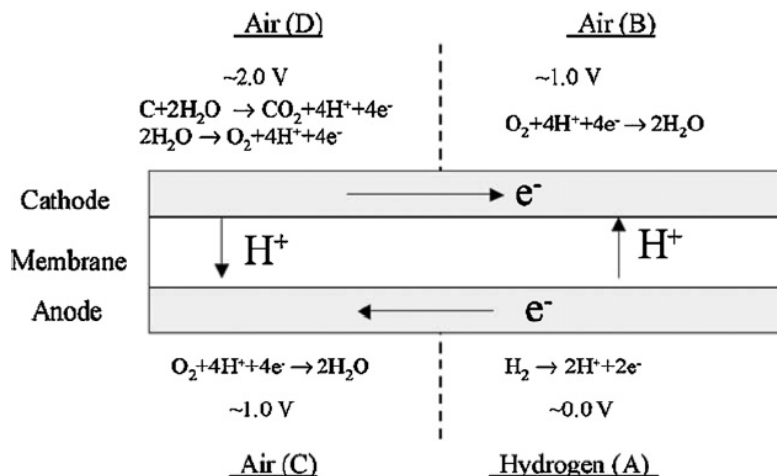
Fig. 2.3 – Schematic of reversal current model (reproduced from [98])
