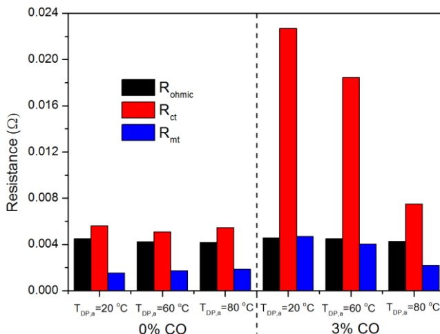
Fig. 4.15 – The corresponding fitted resistances of the fuel cell calculated from the spectra shown in Fig. 4.12.
