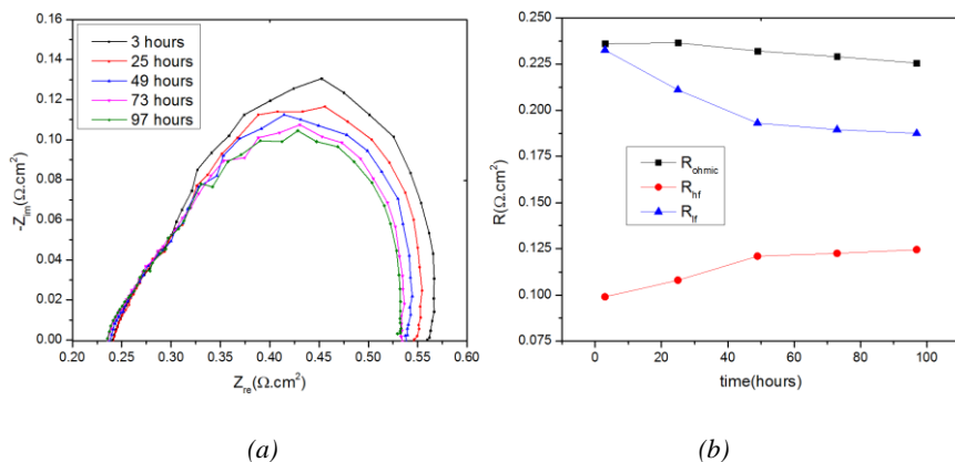
Fig. 4.8 – Evolution of impedance spectra (a) and all the internal resistances (b) of the first fuel cell throughout the H_2 continuous test
