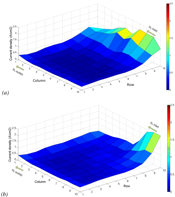
Fig. 4.28 – The current density distribution profile of the fuel cell when the cell reversal occurred and the cell voltage decreased to the lowest level during the H 2 starvation process under the H 2 stoichiometry of 0.4 and current load of 10 A
