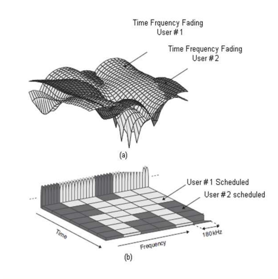
Figure 2.3: Example of time and frequency domain resource allocation using OFDMA [5].
