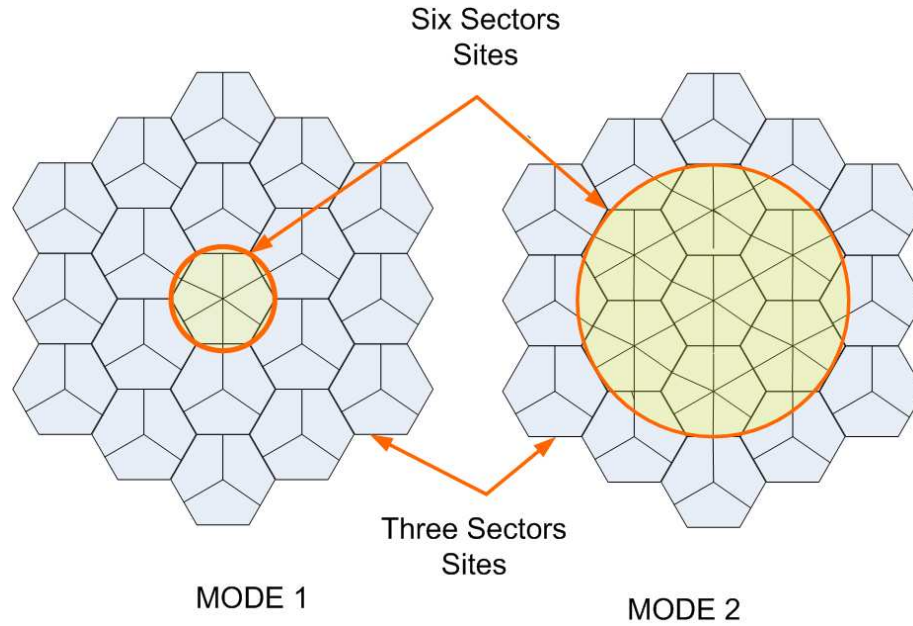
Figure 3.3: Proposed mixed network topologies
