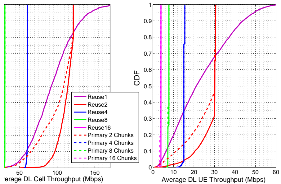
Figure 6.16: CDF of DL cell throughput and user throughput of regular office scenario with random HeNB switching.
