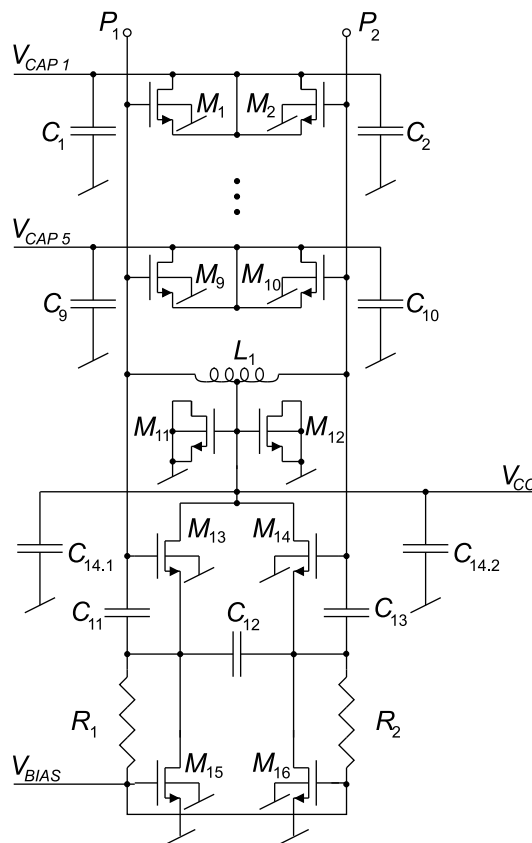
FIGURE 24: Diagram of the implemented Q-enhanced LC resonator.
