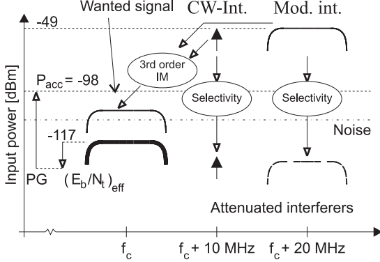
Figure 4: Intermodulation test.
