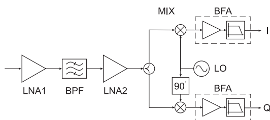
Figure 8: Direct-conversion receiver.
