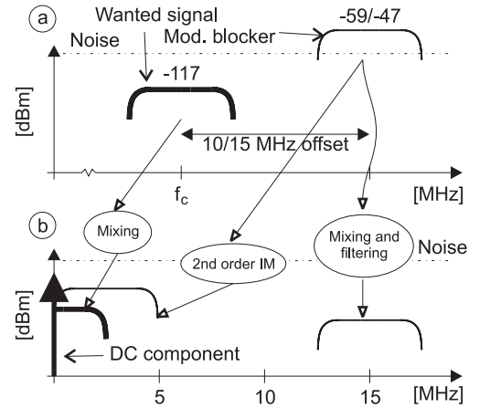
Figure 3: In-band modulated blocker test. (a) RF spectrum with wanted signal and an offset modulated blocker. (b) Baseband spectrum with desired and disturbing signals.
