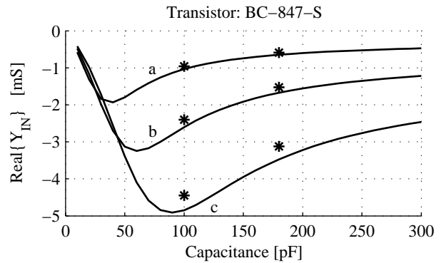
Figure 8: Real part of the input admittance versus capacitance level ( C_1 = C_2 = C_3 ) measured (*) and estimated from Eq. (9) (solid lines) for the BC-847-S transistor. Letters a-c refer to the conditions in Table 2.
