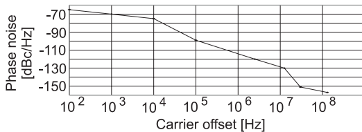
Figure 7: Tx LO phase noise requirement.
