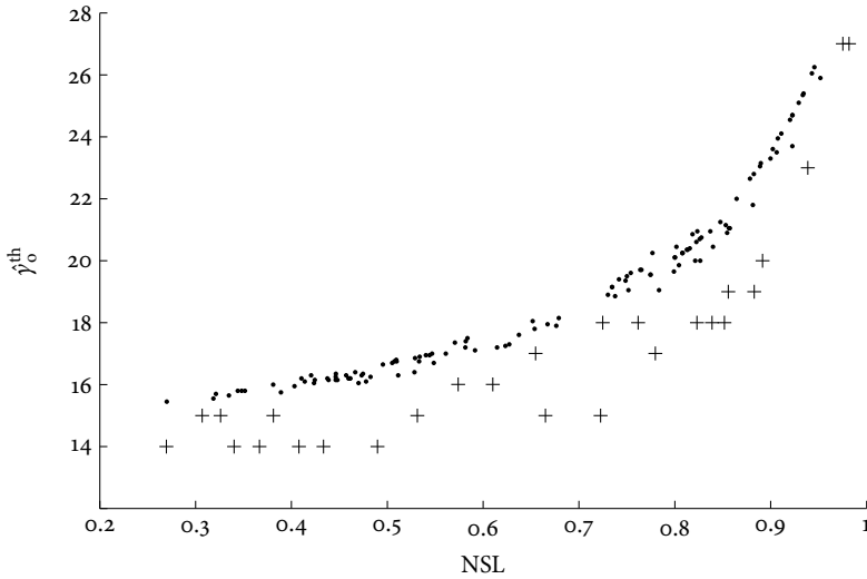
Fig. B.6: The estimated RMSEE threshold \hat{\gamma}_0^{\text{th}} as a function of the NSL. The points marked by \bullet are obtained from the Athley's method, while the points marked with + are obtained from Monte Carlo simulations. The simulation setting is described in the caption of Fig. B.5.
