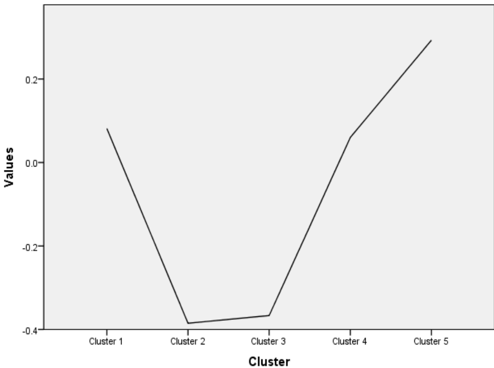
Final Cluster Centers trivsel
