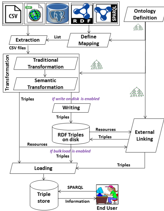
Fig. D.3: SETL architecture.
