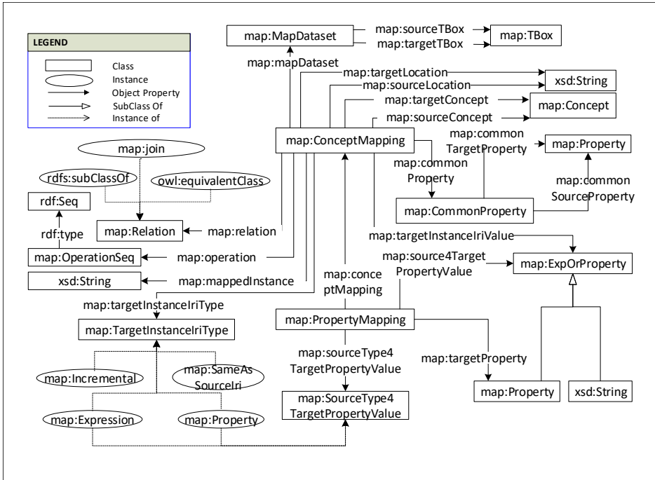
Fig. 9: Pictorial summary of the key terms and their relationship of the S2TMAP vocabulary. (Reproduced from [17])
