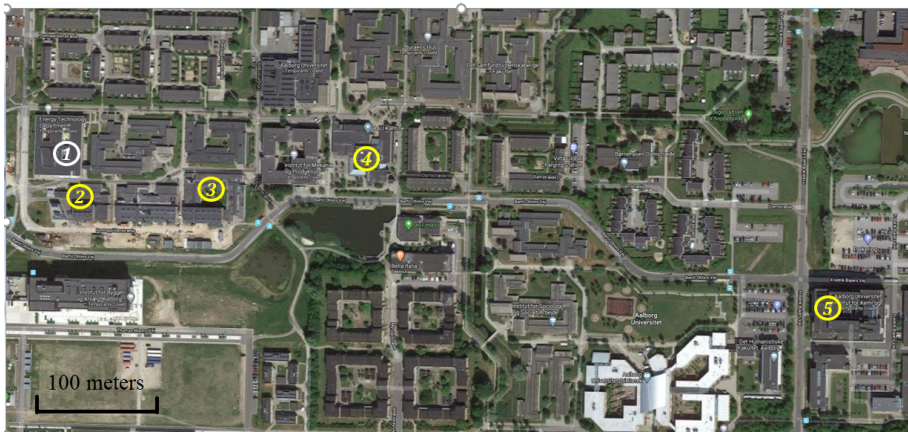
Fig. 4.6: LoRa coverage field test layout. Payload size: twenty bytes - Image source:Google Maps, Aalborg University campus.
