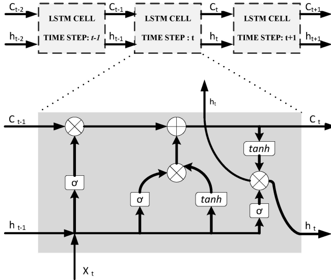
Fig. 5.2: LSTM-RNN
