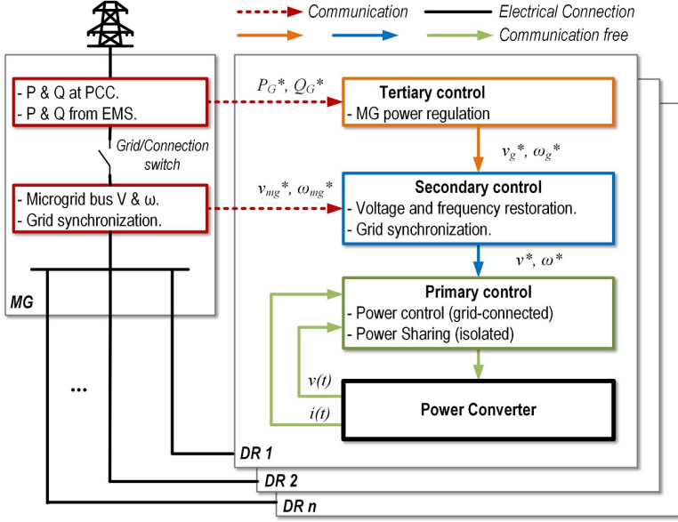
Fig. 1.1: MG control hierarchy.
