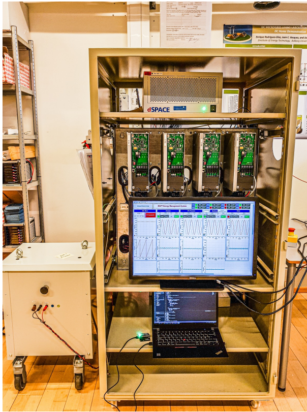
Fig. 3.4: Experimental setup in AC-MG lab, Aalborg University.
