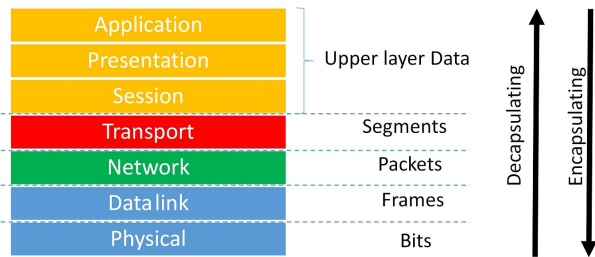
(a) OSI
