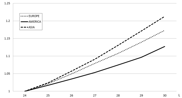
Fig. 3. Cost vs. Number of Links
