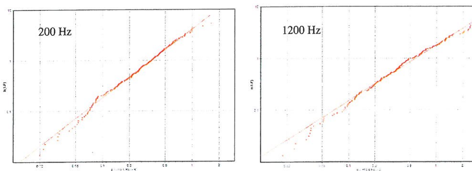
Figure 16. Weibull plot for transducer 14 – test 3 (at 200 Hz and 1200 Hz).
