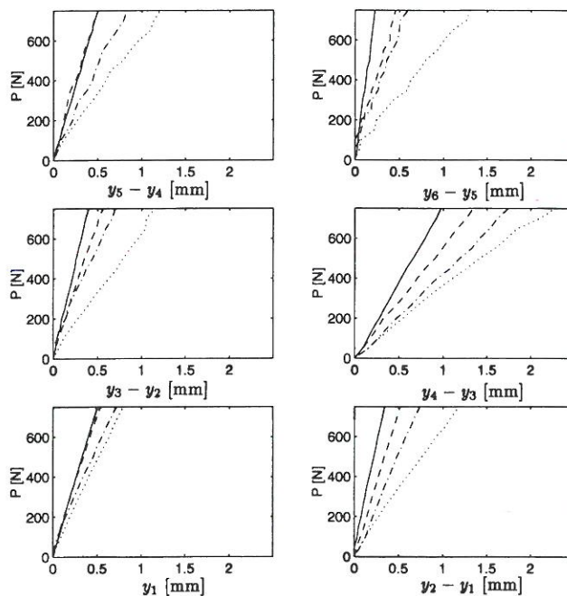
Fig. 16. Force–deformation curves for interstorey displacements obtained from the static tests of the frame: —, virgin structure; ---, after EQ1; - · -, after EQ2; · · · after EQ3.
