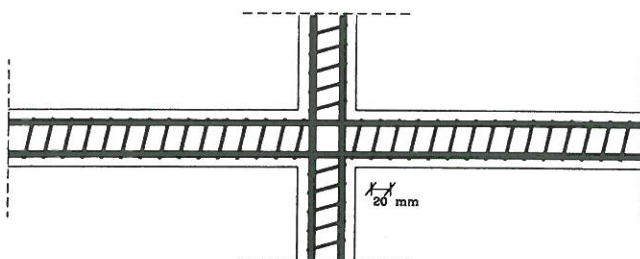
Fig. 4. Shear reinforcement of columns and beams.
