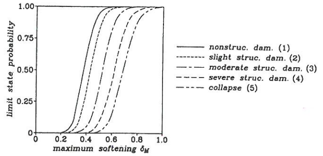
Fig. 14. Distribution function of observed limit state values of one-dimensional maximum softening reported by DiPasquale et al. 5
