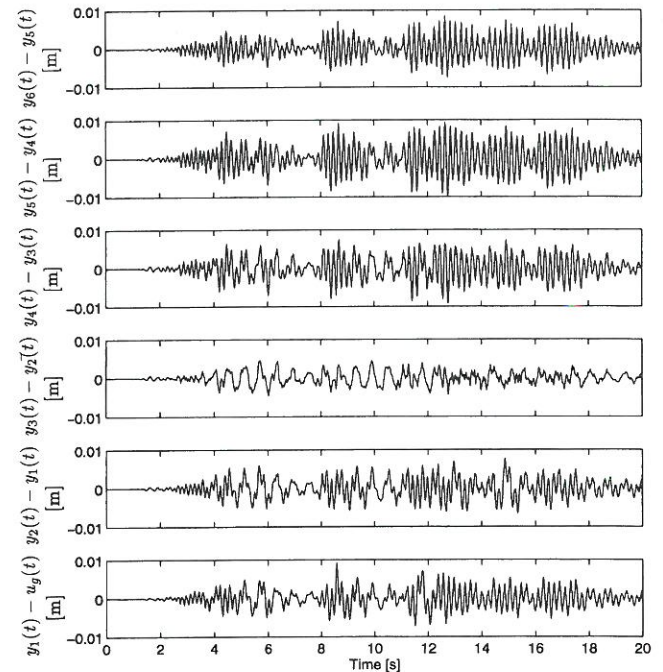
Fig. 11. Interstorey displacements during EQ2 for frame AAU4.
