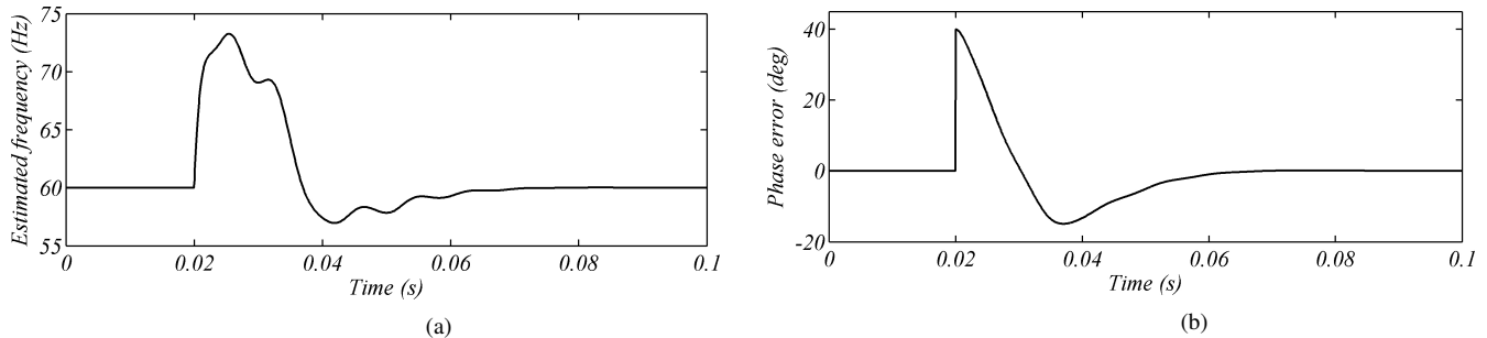
Fig. 15. Simulation results for the phase jump of 40^\circ : a) estimated frequency, b) phase error.
