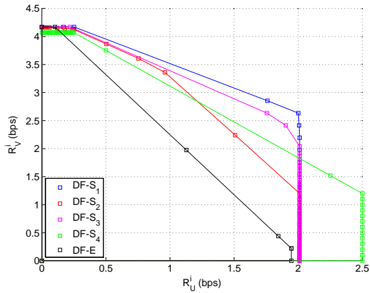
Fig. 8. Rate region of (R_U^i, R_V^i) ( i \in \{S_1, \dots, S_4, E\} ) for DF CDR and reference schemes.
