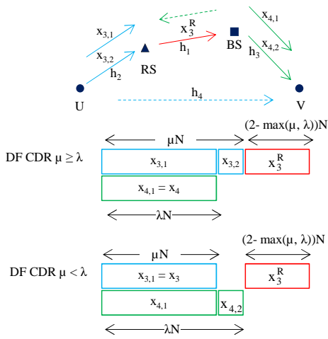
Fig. 2. Time slots in CDR Scheme S_2 .
