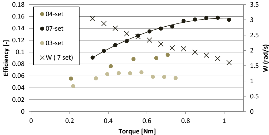
Figure 19. Efficiency for different number of fin's sets depending on torque values under wave condition \emptyset (RW \emptyset ). 0.75mm, 6 fins par set, draft=0.36m. Average measured H=0.15 m, T=1.4 s.
