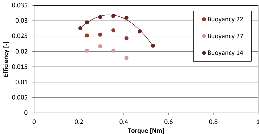
Figure 30. Efficiency depending on the torque for different buoyancy levels, 4 sets of fins, 6 fins par set with 1 mm thickness.
