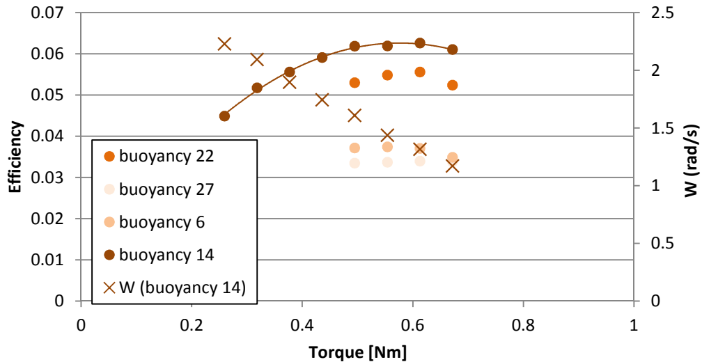
Figure 29. Efficiency depending on the torque for different buoyancy levels, 7 sets of fins, 6 fins par set with 0.75 mm thickness.
