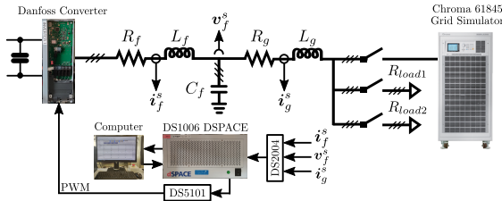
Fig. 8. Experiment setup.
