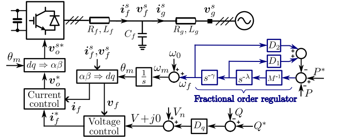
Fig. 1. FOVSG circuit and block diagram.
