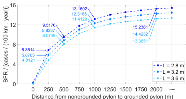
Fig. 11. Effect of increasing insulation distance L on BFR of different PGTLs distances
