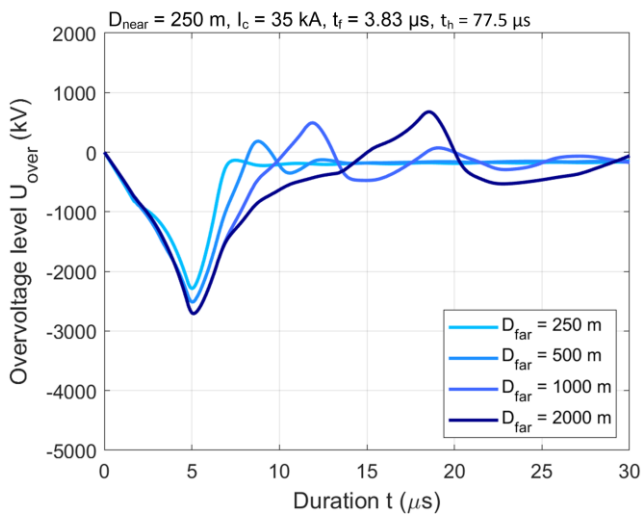
Fig. 6. Overvoltage wave fronts of same D_{near} and different D_{far}
