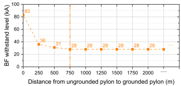
Fig. 8. BF withstand level of different distances to nearest grounded pylon
