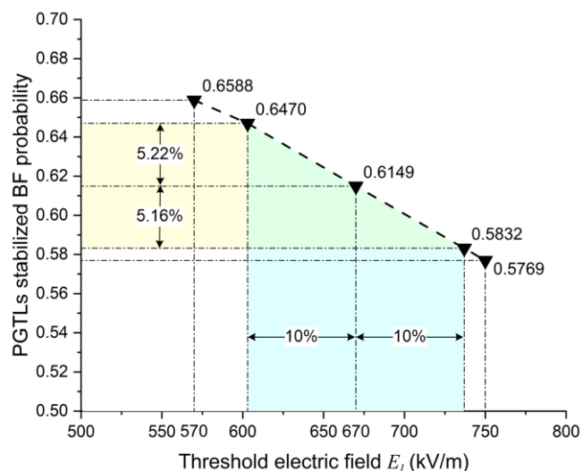
Fig. 12. Sensitivity analysis result of PGTLs stabilized BF probability to the threshold electric field E_l
