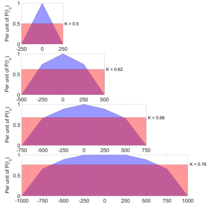
Fig. 13. Demonstration of the BF probability unitization and estimation of K
