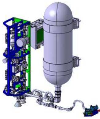
Figure 6. Rendering of the PROP system; Propellant tank with pressure management system and one thruster cluster shown
