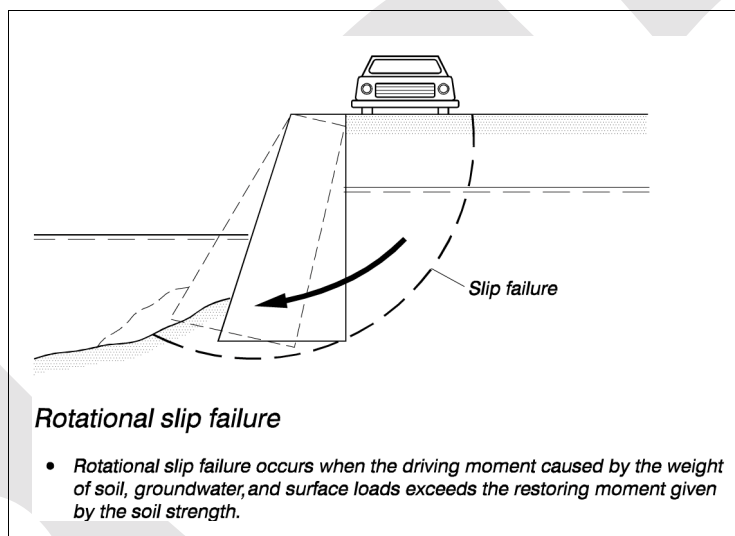
Figure VI-2-66. Rotational slip failure of gravity wall
