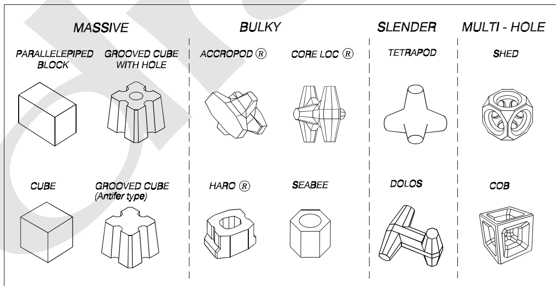
Figure VI-2-24. Examples of concrete armor units
