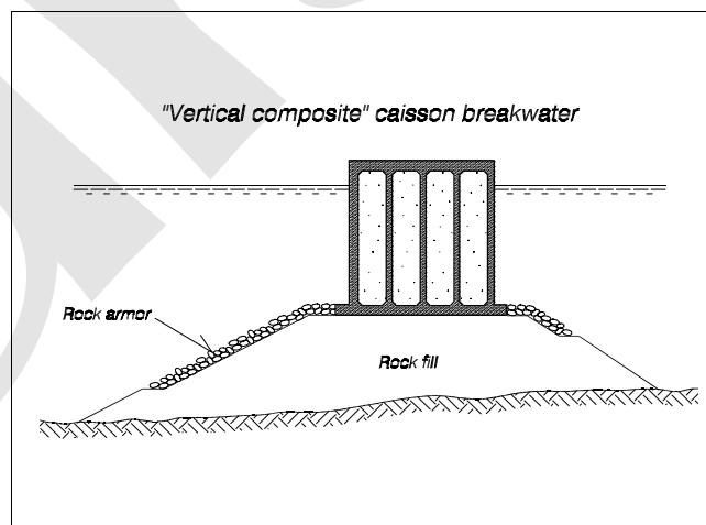
Figure VI-2-17. Vertical composite caisson breakwater
