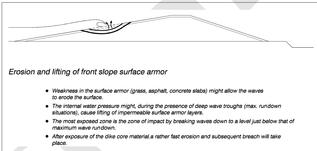
Figure VI-2-47. Erosion of dike slope protection
