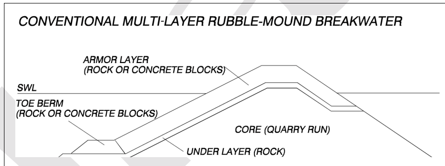
Figure VI-2-11. Conventional multilayer rubble-mound breakwater
