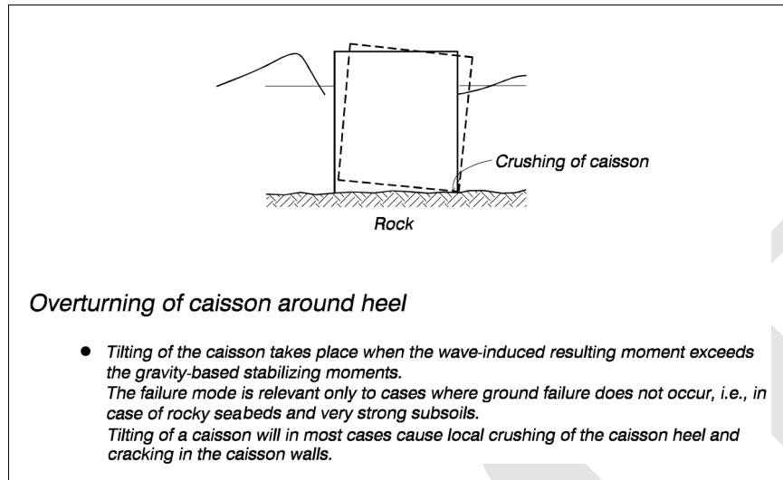
Figure VI-2-56. Caisson overturning
