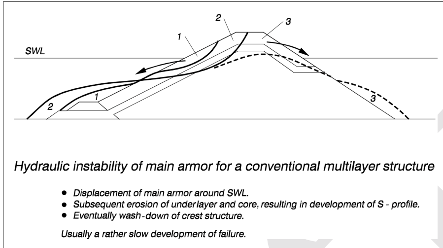
Figure VI-2-26. Main armor layer instability
