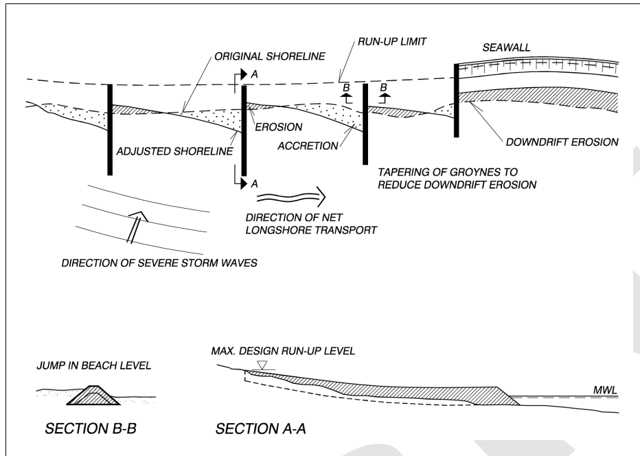
Figure VI-2-8. Typical beach configuration with groins
