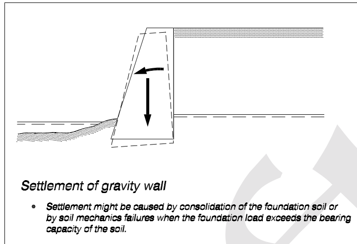
Figure VI-2-65. Gravity wall settlement
