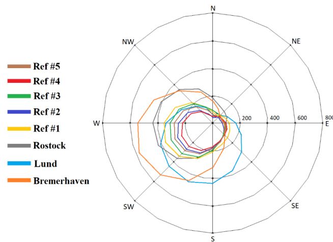
Figure 4. Total amount of wind driven rain in relation to orientation. Produced in WUFI® Pro.
