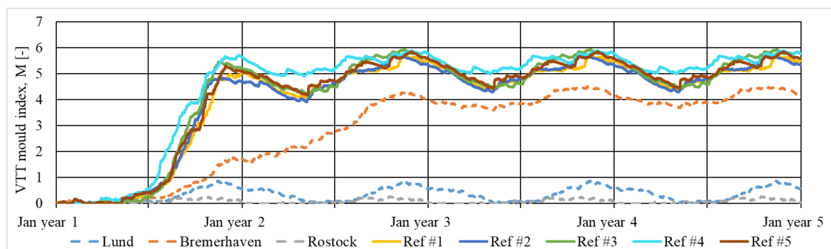
Figure 6. VTT mould growth predictions for wood exposed to the climatic conditions of the generated moisture reference years, and comparison with Lund, Bremerhaven, and Rostock.
