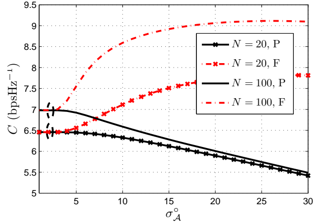
Fig. 11. Capacity performance versus the angle spread of the cluster when partial (P) and full (F) CSI is available at the BS. The performance is shown for two ULAs of 20 and 100 isotropic antenna elements.
