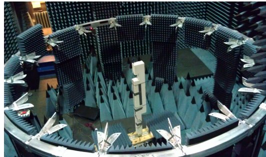
Figure 1. Practical anechoic chamber setup in the measurement system
