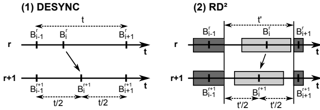
Fig. 1: DESYNC and RD^2 beacon time calculation
