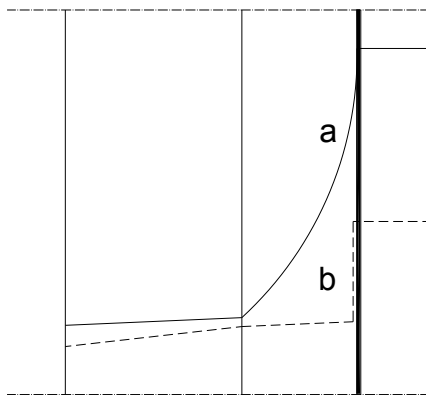
Fig. 1b. Vapour pressure distribution, PE-foil. a. Saturated vapour pressure b. Actual vapour pressure (no interstitial condensation)
