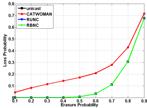
Fig. 2. The analytical result of loss probability.
