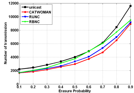
Fig. 5. Simulation result for the expected number of transmission.
