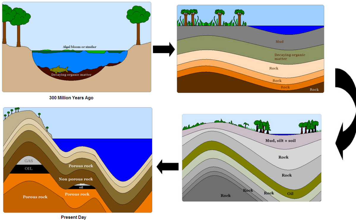
Figure 26: Formation of fossil fuels [22].
