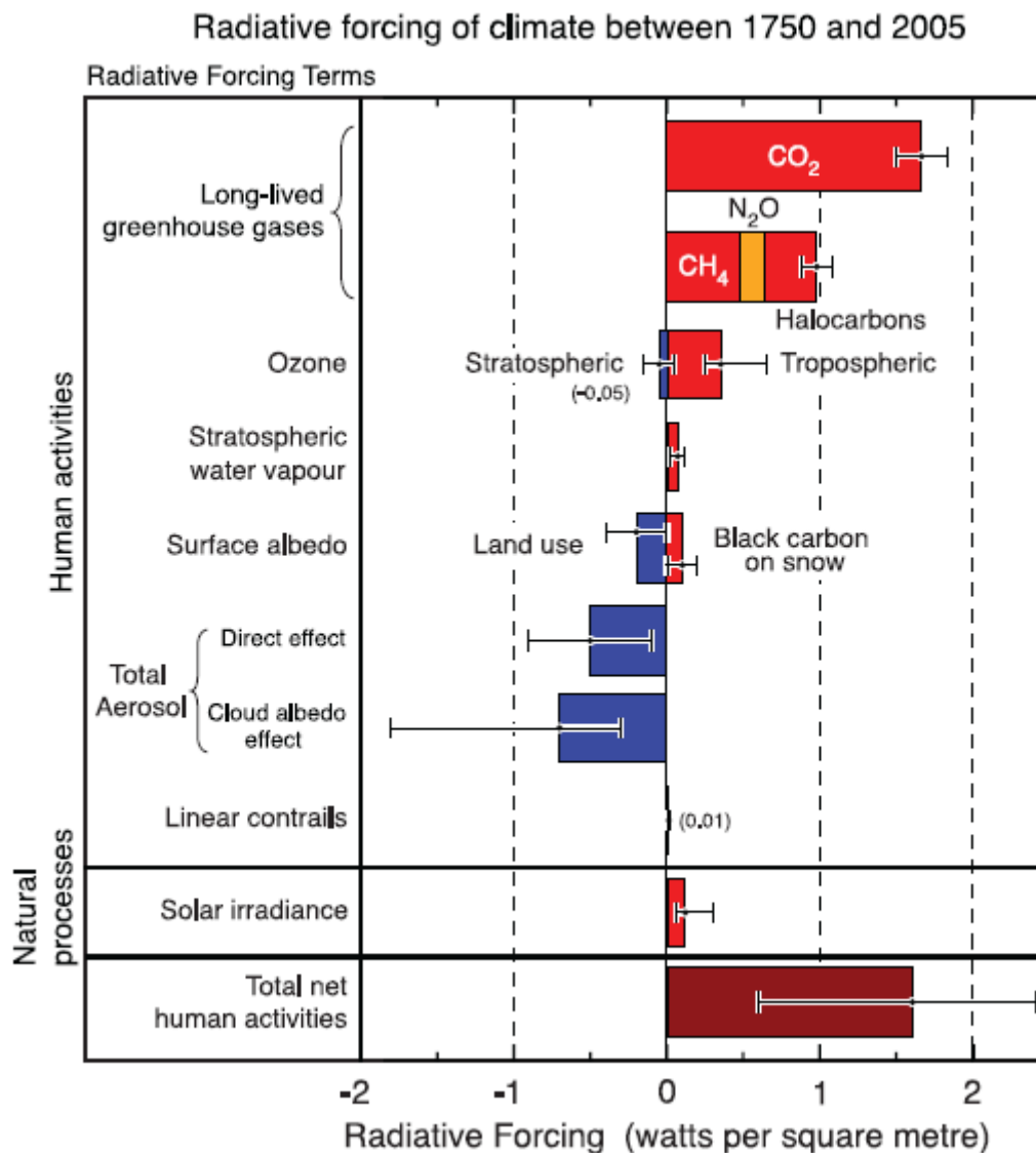
Figure 2: Principal components of the radiative forcing causing climate change between 1750 and 2005 [3].
