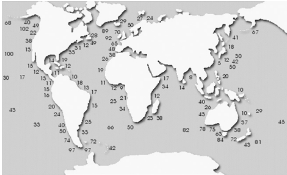
Figure 30: Estimated global wave energy power in kW [23].
