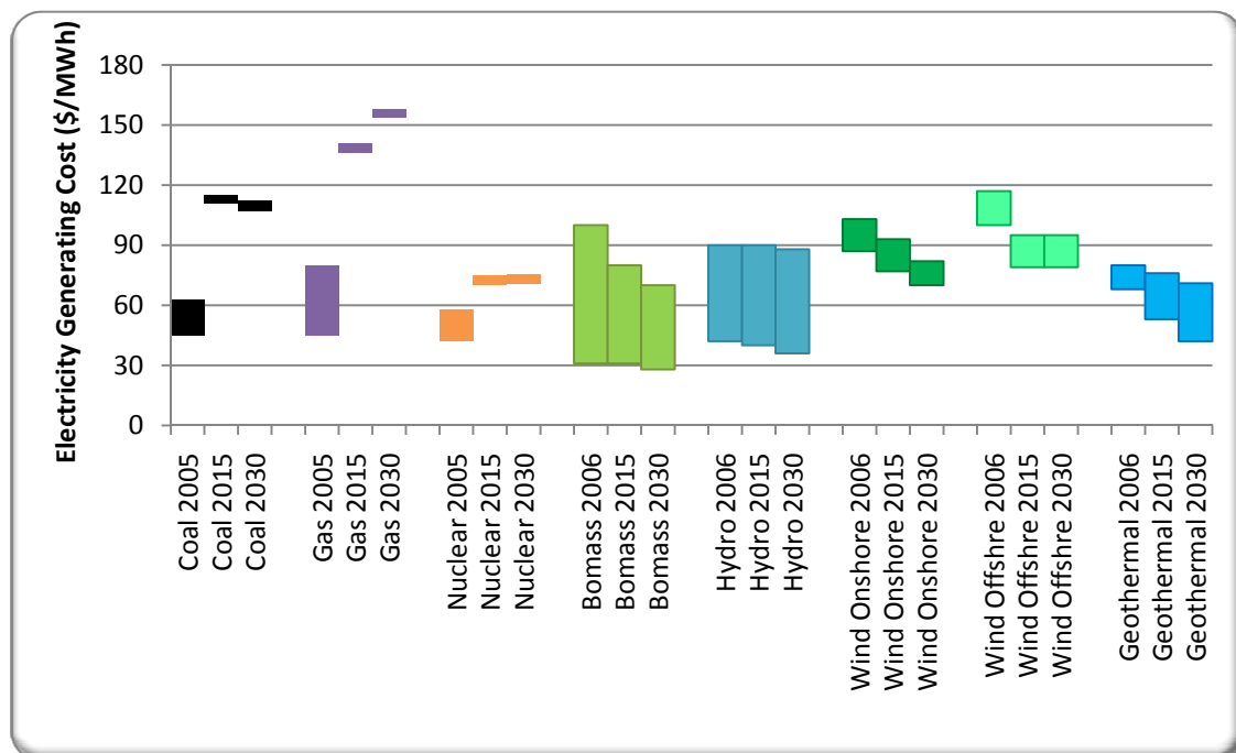
Figure 24: Current cost of renewable and fossil fuel based electricity production along with projected costs for 2015 and 2030 [19-21].
