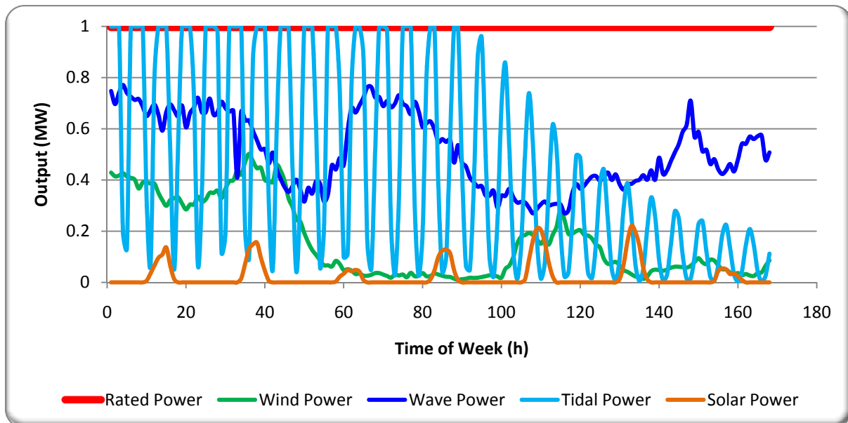
Figure 28: Predicted hourly output from a wind, wave, tidal, and solar electricity generator in Ireland during week 1 of January 2007.
