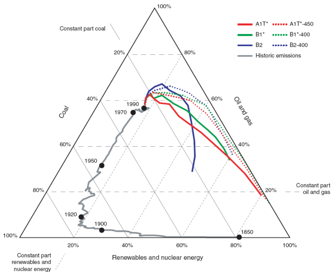
Figure 20: Evolution of energy consumption from 1850 to 1990, with various projections up to 2100 [14, 15].
