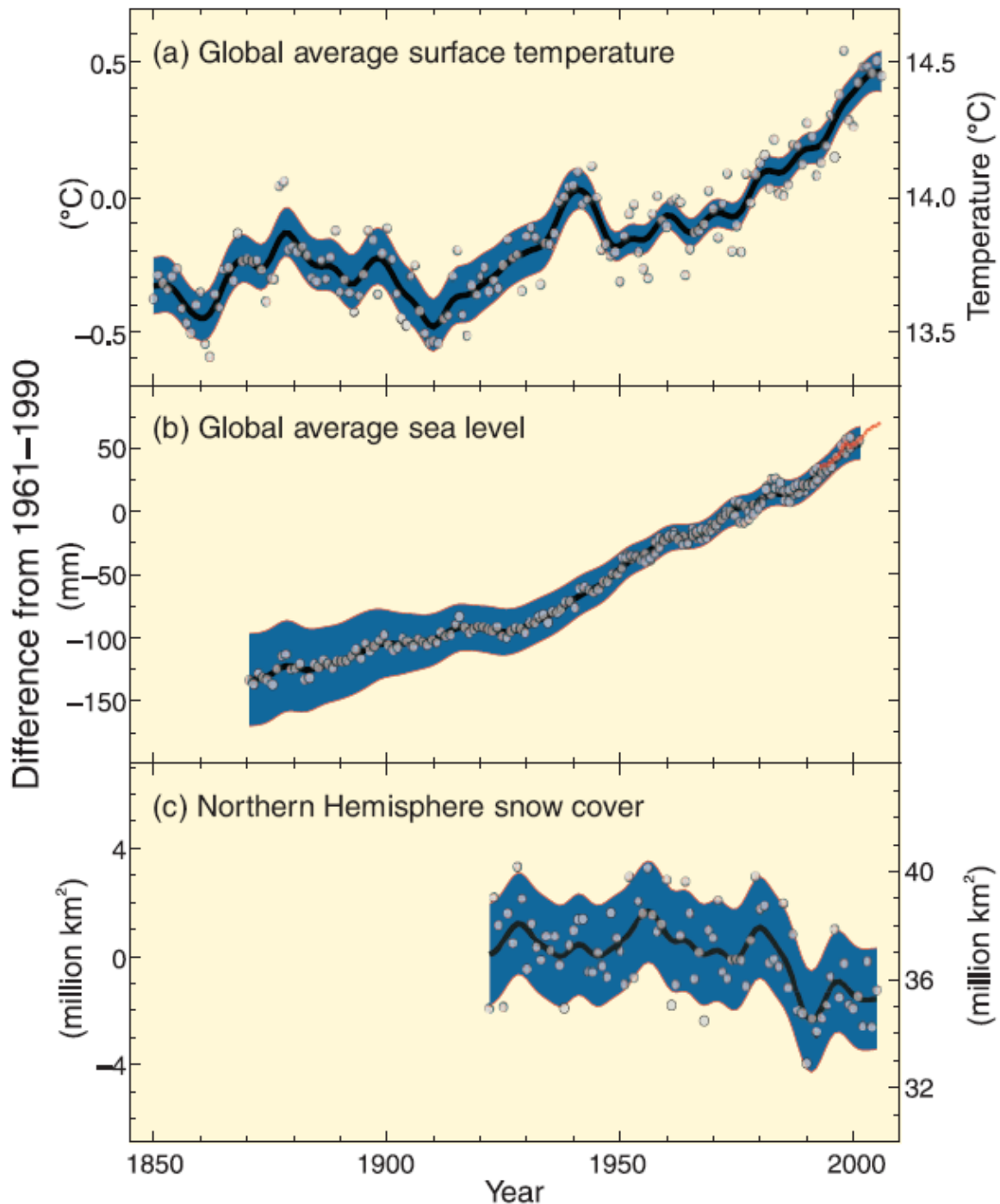
Figure 4: Observed changes in (a) global average surface temperature; (b) global average sea level from tide gauge (blue) and satellite (red) data; and (c) Northern Hemisphere snow cover for March–April. All differences are relative to corresponding averages for the period 1961–1990 [5].
