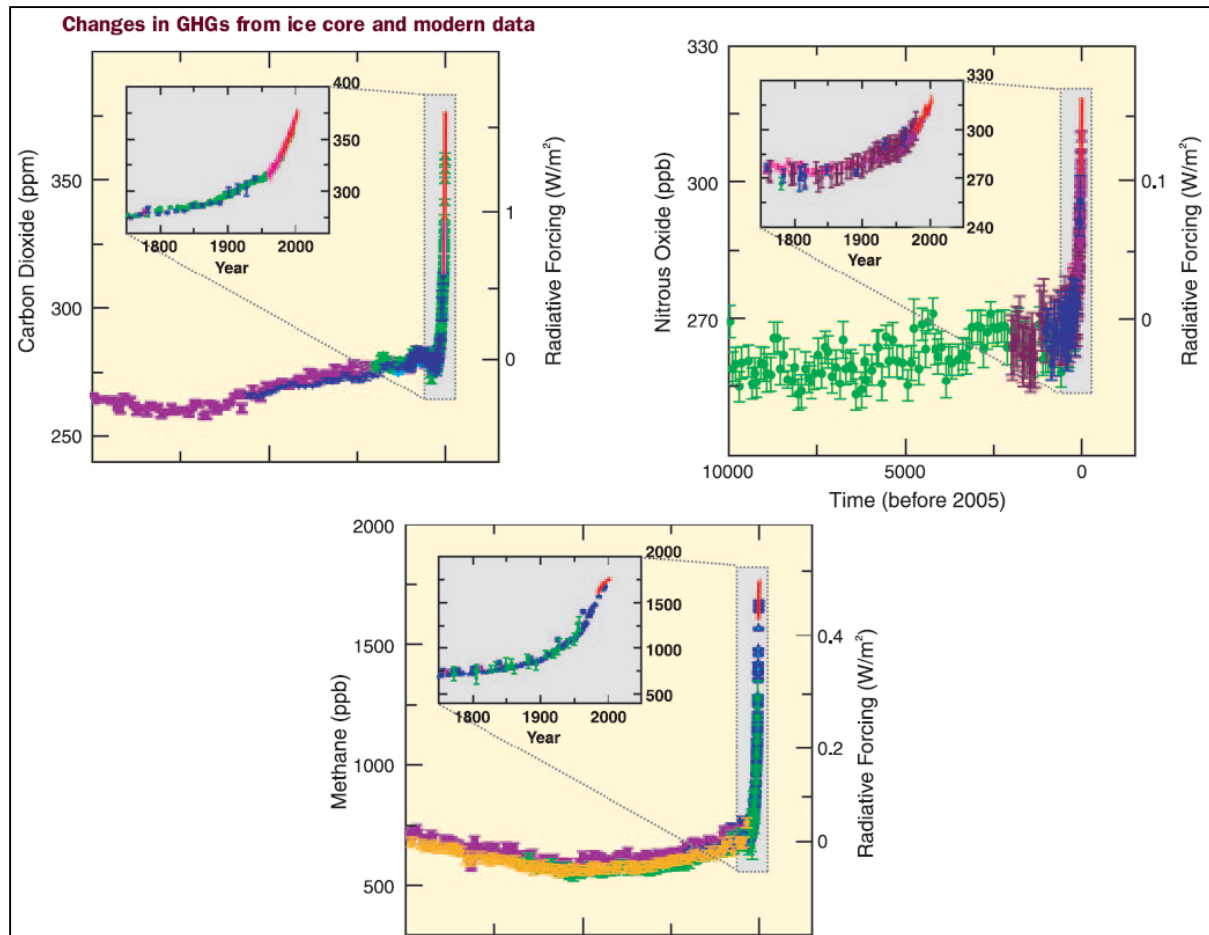
Figure 3: Concentration of \text{CO}_2 , \text{CH}_4 , and \text{N}_2\text{O} in the earth's atmosphere over the last 10,000 years [4].
