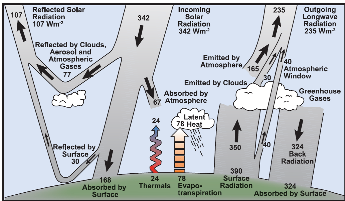
Figure 1: Estimate of the earth's annual and global mean solar radiation balance.
