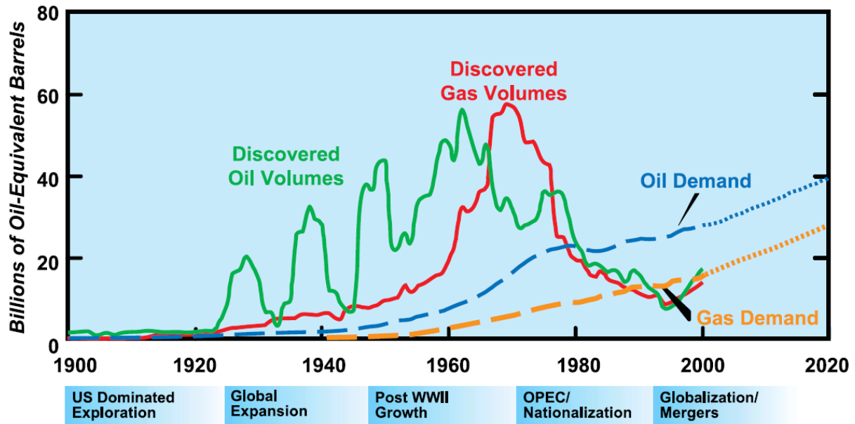
Figure 12: Historical discovery and consumption of fossil fuel [12].
