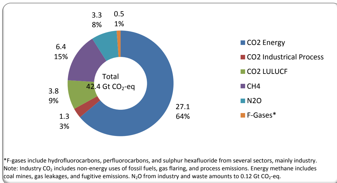
Figure 6: World anthropogenic greenhouse-gas emissions quantified by CO 2 equivalent and divided by source for the year 2005 [6].
