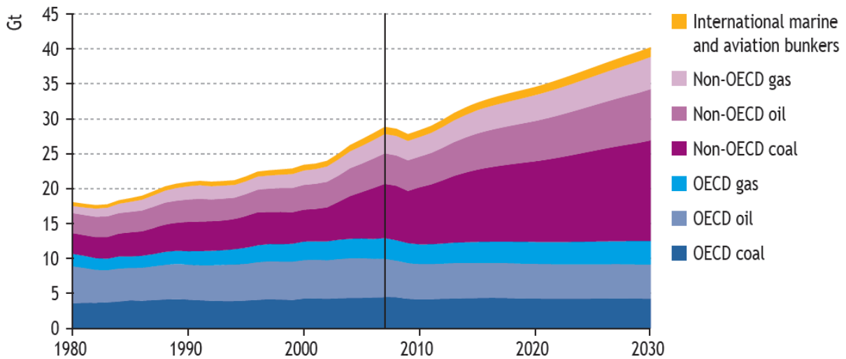
Figure 10: Historical and projected global CO 2 emissions due to energy [6].
