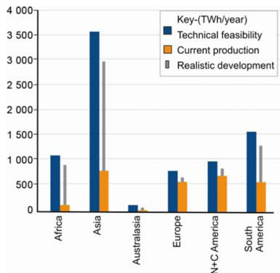
Figure 27: Global hydro resource that has been utilised and that is feasible in the future [23].
