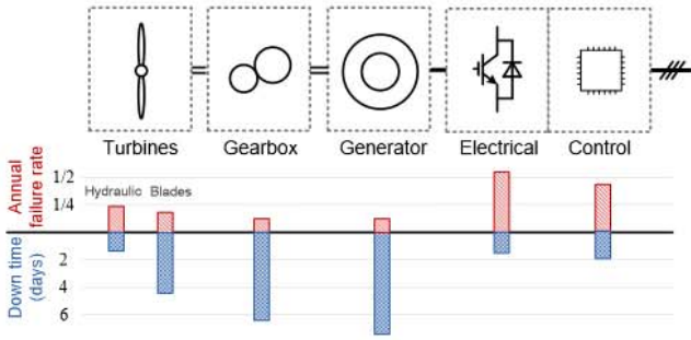
Fig. 19. Wind turbine overview in respect to reliability where registered annual failure rate and down time are illustrated. Data from [46].
