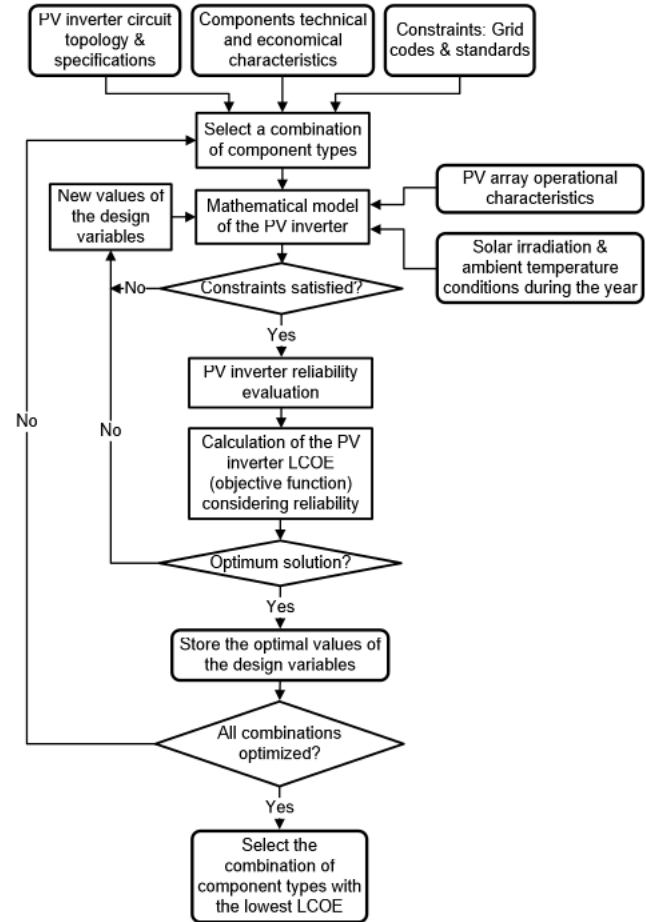
Fig. 2. A flow-chart of the proposed optimization procedure.
