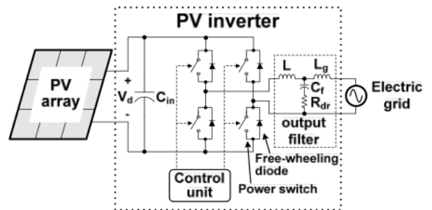
Fig. 1. A grid-connected PV system employing a transformerless PV inverter.
