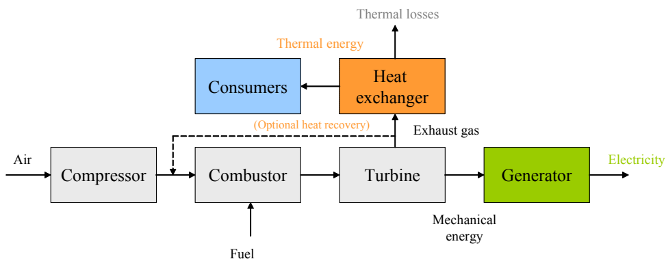
Figure 8-3: Micro gas turbine components
