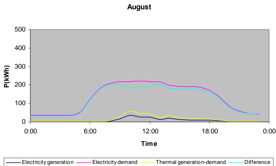
Figure 5-30: Amount of electricity imported form/exported to the market on a summer day
