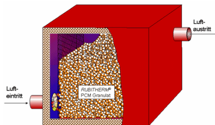
Figure 11-12: Air-reservoir with PCM /Rubitherm/
