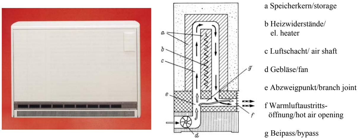
Figure 9-1: STIEBEL ELTRON storage heater, view from outside. Typical modern type, /1/
