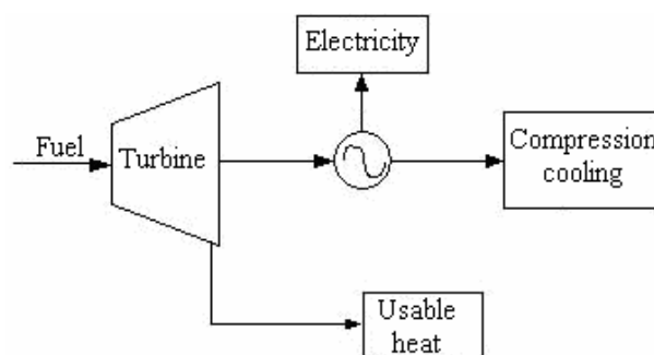
Figure 5-3: Trigeneration with compression chiller
