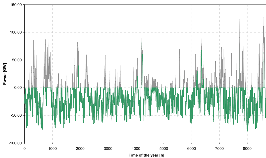
Figure 3-28: Scenario IV: Balanced with contribution of Demand Side Management
