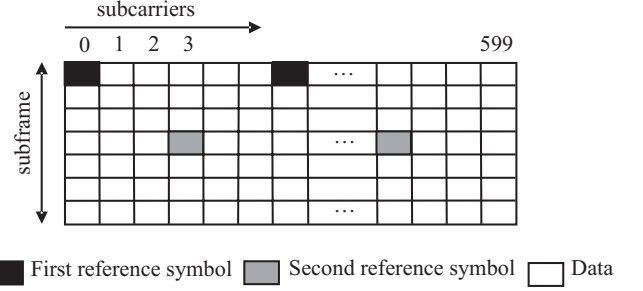
Figure 3: Downlink reference-signal structure for UTRAN LTE [1]
