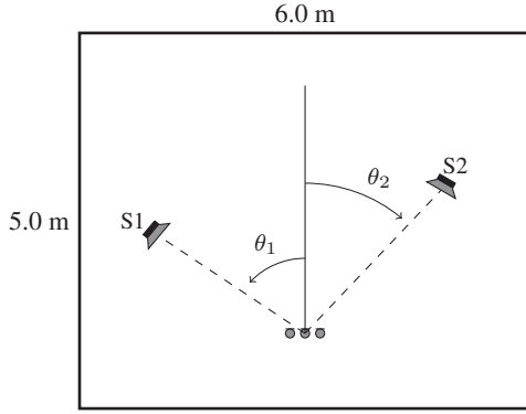
Fig. 2. The room layout and the azimuth angles of sound sources; \theta_1 \approx -53^\circ and \theta_2 \approx 45^\circ
