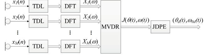
Fig. 1. General diagram of the frequency-domain MVDR beamformer to joint DOA and pitch estimation (JDPE)
