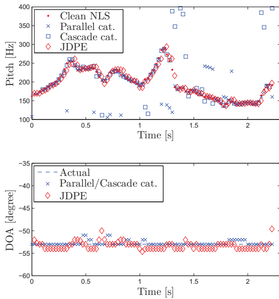
Fig. 4. Estimation of pitch (top), and DOA (bottom) at the different experiments
