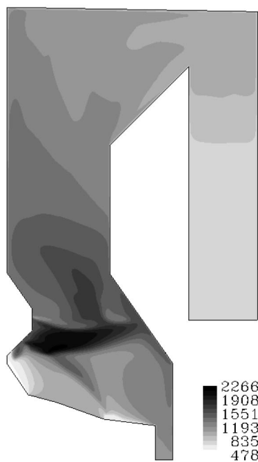
(b) Gas temperature [K]
