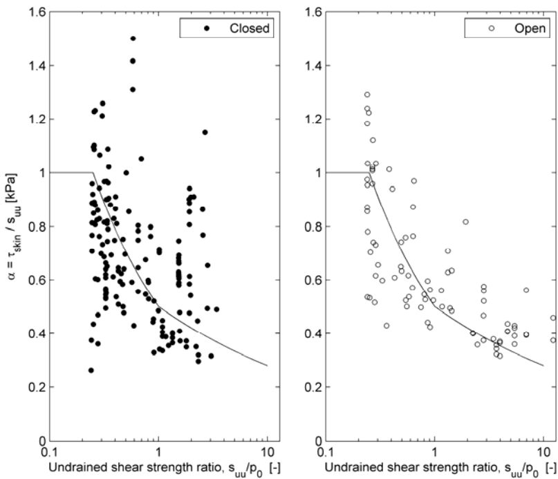
Figure 3. Back-calculated \alpha -values for piles driven closed-ended (to the left) and open-ended (to the right). The solid line describes the relation between \alpha and the undrained shear strength ratio according to API (1993).
