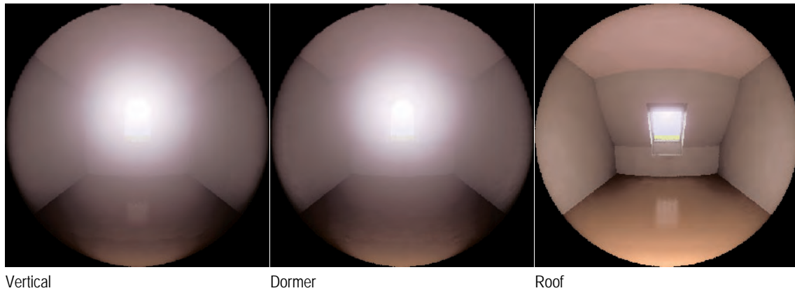
Figure 58. Fish-eye rendering of view toward the window wall under sunny sky conditions in December at 12:00 hours. The images show that the sunlight comes directly into the field of view in all three cases. For the roof window however, the sunlight seems to cause less glare problems.
