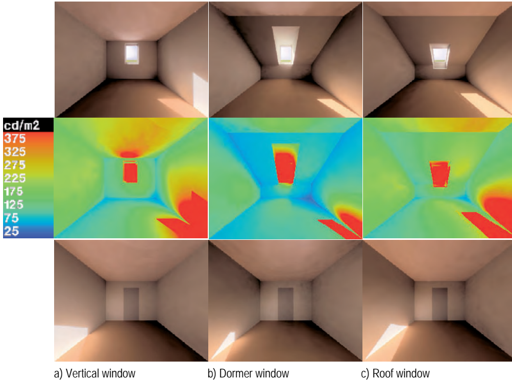
Figure 40. Luminance distribution under sunny sky in March, 10:00. With the vertical window a major part of the sunlight patch fell on the sidewall. For the dormer window the corresponding part of the direct sunlight was on the window linings, while for the roof window the sunlight patch was almost entirely on the floor.
