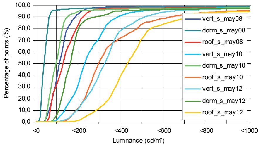
Figure 49. Cumulative frequency distribution of the luminances in the view towards the window, South orientation, sunny day in May at 8:00, 10:00 and 12:00 hours.
