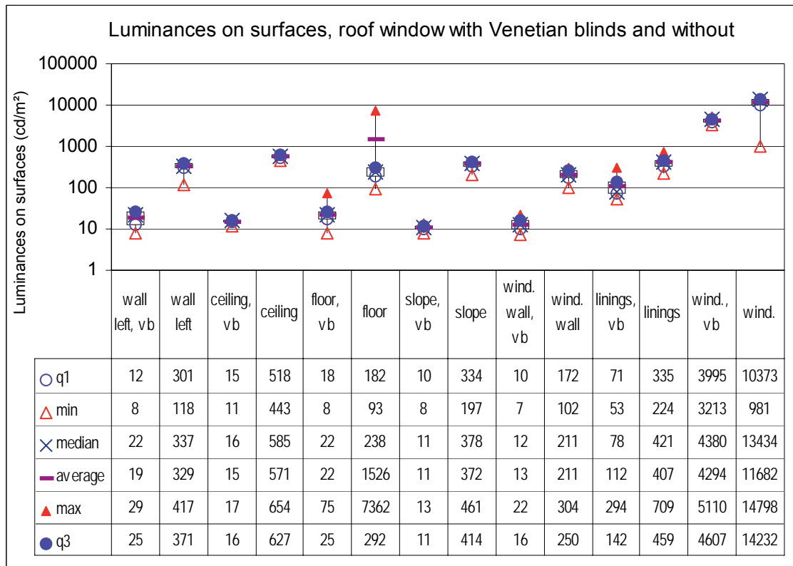
Figure 92. Luminance distribution on surfaces in the room with roof window. Minimum, maximum, median, mean and interquartile range (q1, q3) for luminances ( \text{cd/m}^2 ) of surfaces in the view towards the window wall, under sunny sky conditions in March at 12:00 hours.
