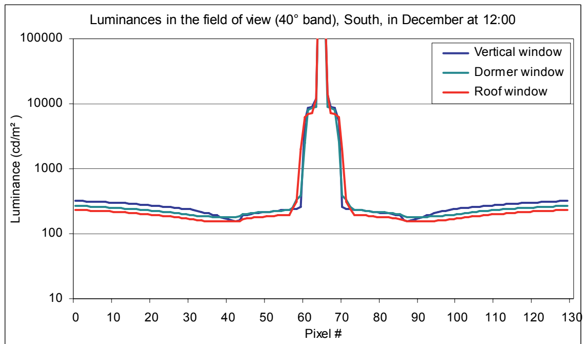
Figure 59. Average luminance within a 40° band centred around the observer's eye looking straight ahead towards the window, under sunny sky conditions, in December at 12:00 hours. The graphs show that because of the direct sunlight penetrating to the back of the rooms in all three cases, the general luminance levels are about the same.
