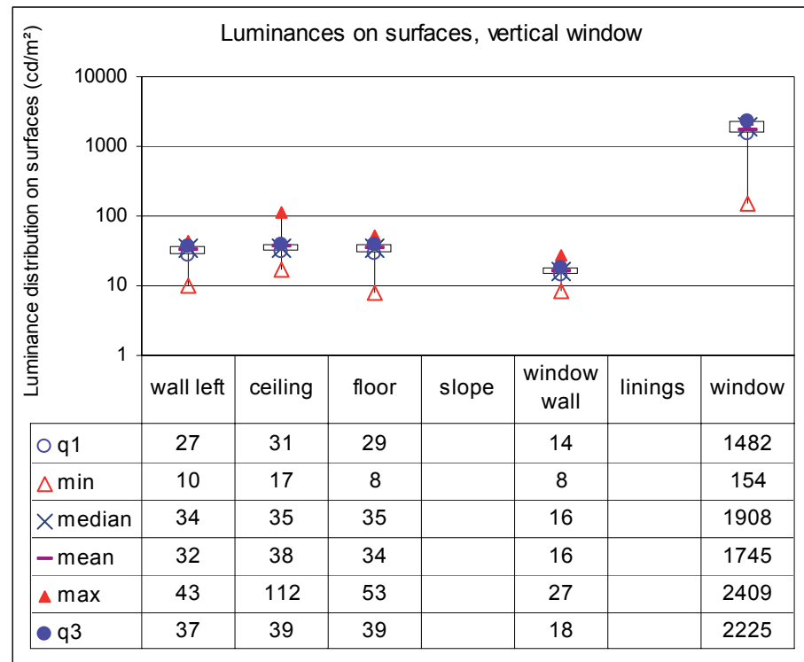
Figure 35. Vertical window. Minimum, maximum, median, mean and interquartile range (Q1, Q3) for luminances ( \text{cd/m}^2 ) of surfaces in the view towards the window wall, under overcast conditions.
