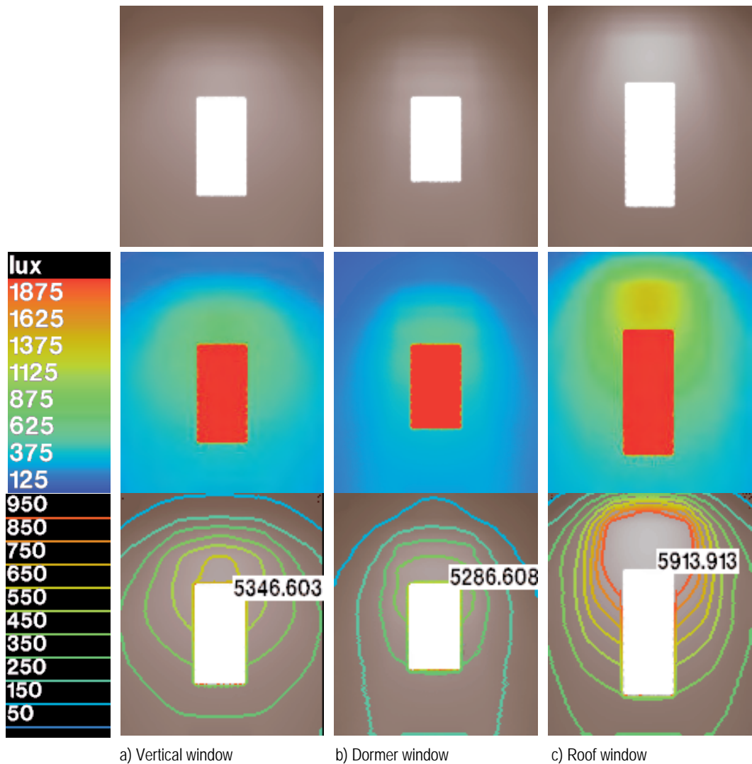
Figure 9. Renderings of a horizontal plane at 0.7 m above floor level, false colour rendering and isolux contours showing illuminance (lux) for the a) vertical, b) dormer, c) roof windows, under intermediate sky conditions oriented South (21 March at 12:00 hours).
