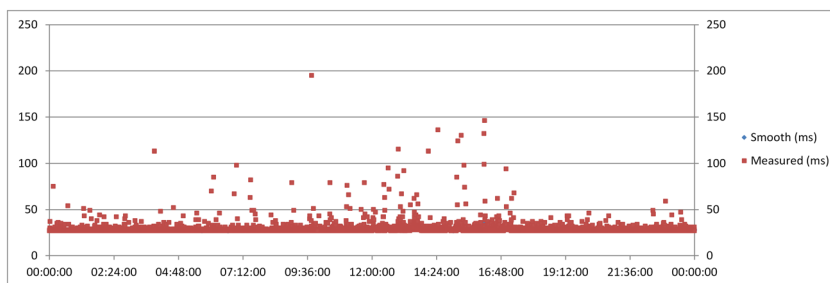
Figure 12. Real and smoothed ping measurements for the first experiment between Aalborg University and the server in Poland.
