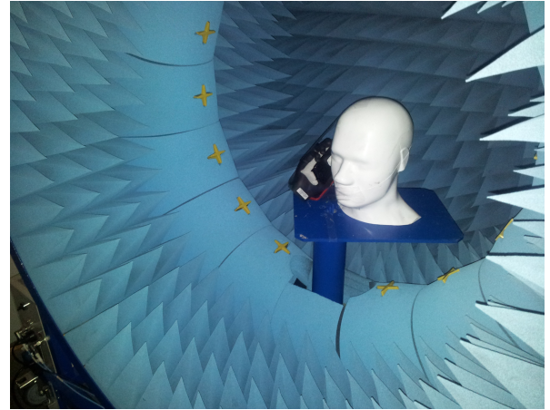
Fig. 2. Illustration of the SAM and hand phantom placement in the Starlab chamber for obtaining the TRP and TIS results.
