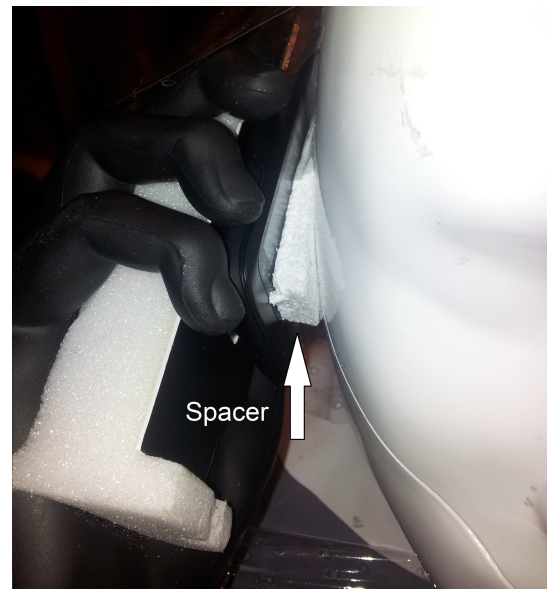
Fig. 3. Close up of the phone's placement on the phantom's cheek.
