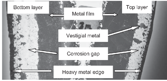
(a) Separation of metal film from heavy edge by corrosion.
