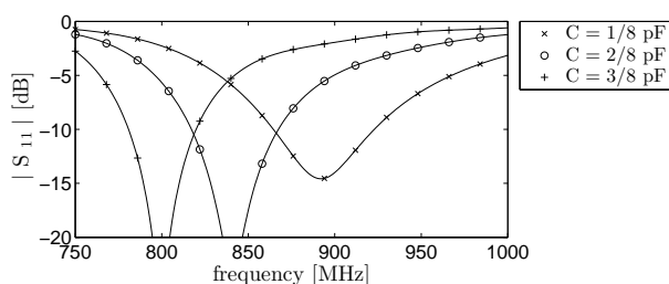
Fig. 2 Tuning range of the low-Q antenna (A1)
