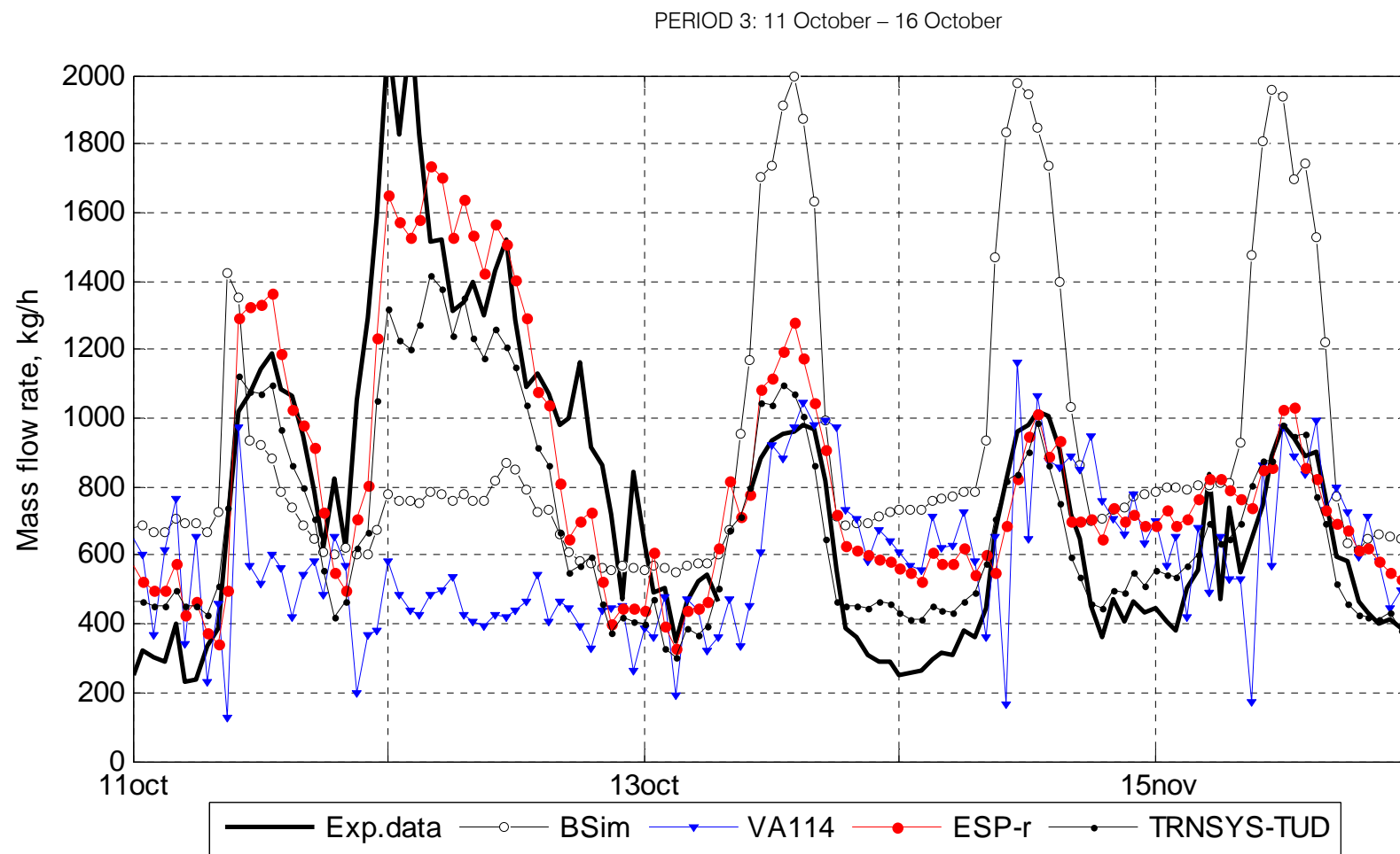
Figure 68. Hour averaged mass flow rate in the zone 1, measured with the tracer gas method (PERIOD 3: 11 October – 16 October).
