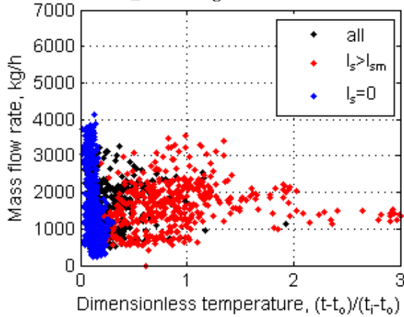
Figure 8. Correlation between dimensionless air temperature in the DSF cavity and mass flow rate in the cavity.
