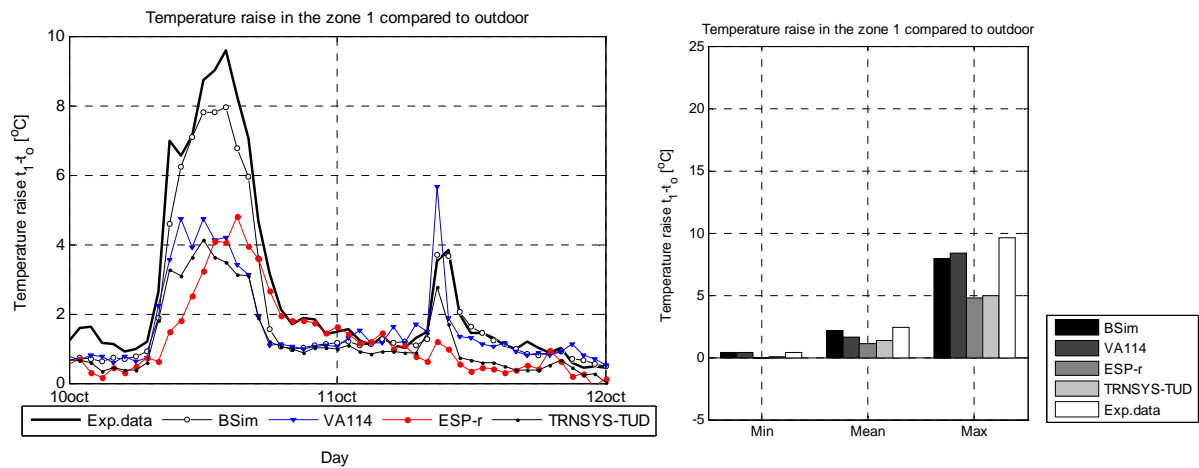
Figure 57. Temperature raise in the zone 1 compared to outdoor. Test case DSF200_e.
