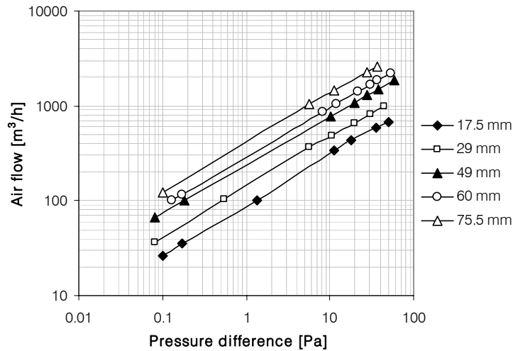
Figure 26. Correlation between pressure difference and air flow rate through the window for different opening angles obtained for point 1.
