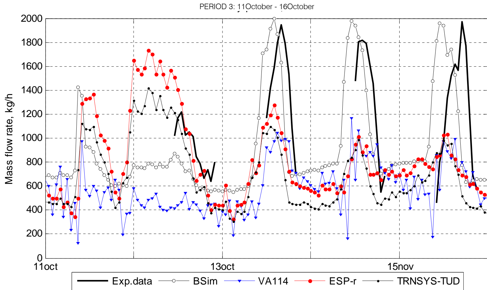
Figure 71. Hour averaged mass flow rate in the zone 1, measured with the velocity profile method. Velocity profile at h=1.91\text{m} (PERIOD 3: 11 October – 16 October).
