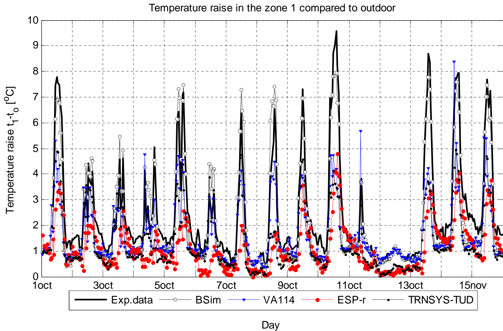
Figure 58. Temperature raise in the zone 1 compared to outdoor. Test case DSF200_e.
