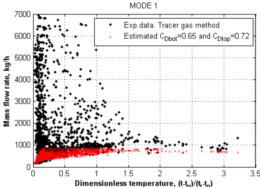
Figure 10. Estimated mass flow rate in the DSF cavity for pure buoyancy natural ventilation.
