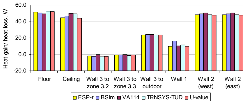
Figure 18. Heat fluxes in the zone 2. Steady State case.
