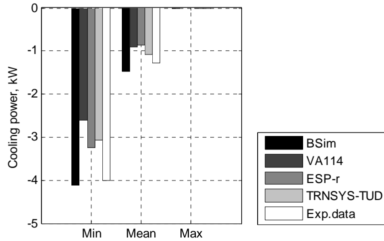
Figure 76. Cooling/heating power in the zone 2. Test case DSF200_e.
