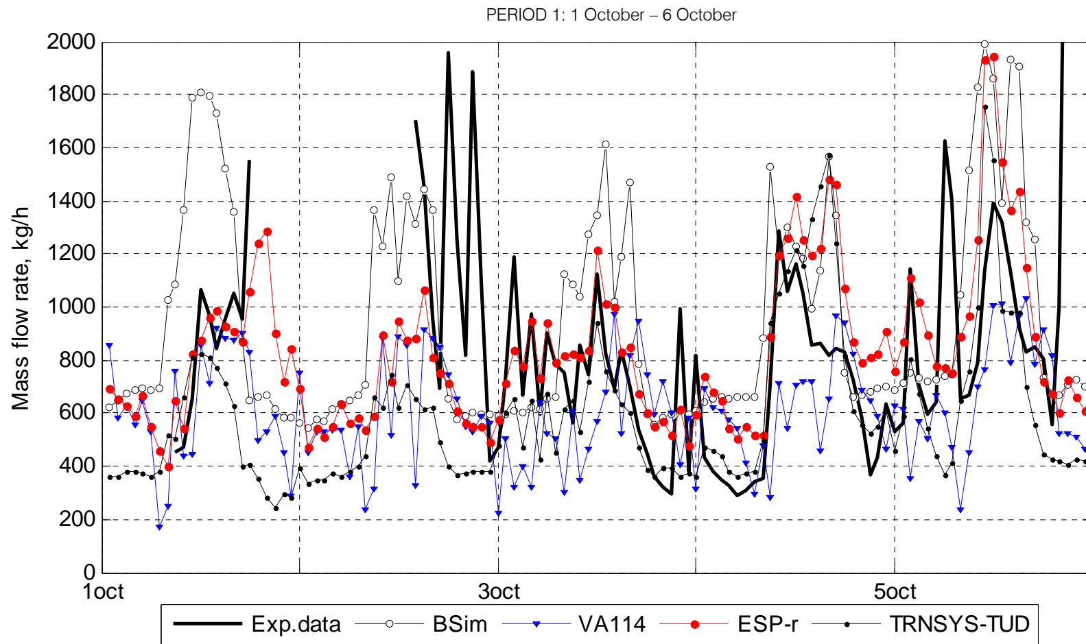
Figure 66. Hour averaged mass flow rate in the zone 1, measured with the tracer gas method (PERIOD 1: 1 October – 6 October).
