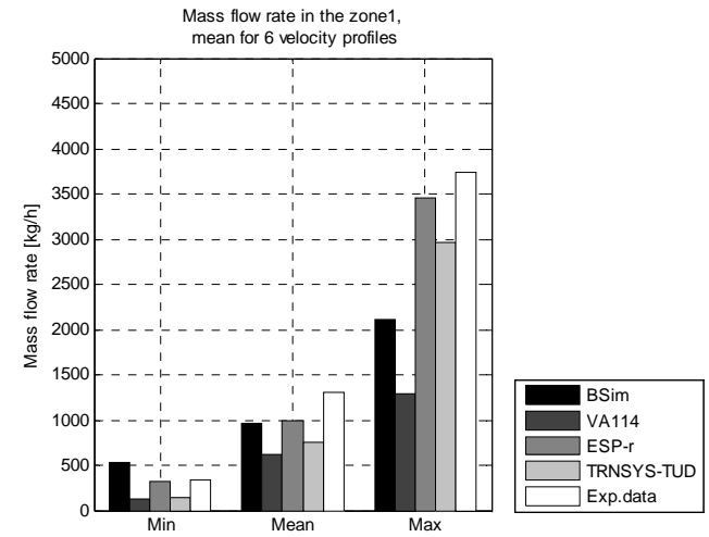
Figure 63. Predicted and measured mass flow rate in the zone 1, measured with the tracer gas method (left). Measured with the velocity profile (right).
