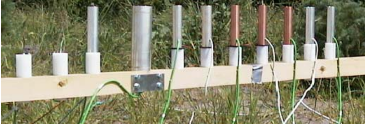
Figure 6. Experimental setup: testing of shielding techniques for air temperature measurements under direct solar access.
