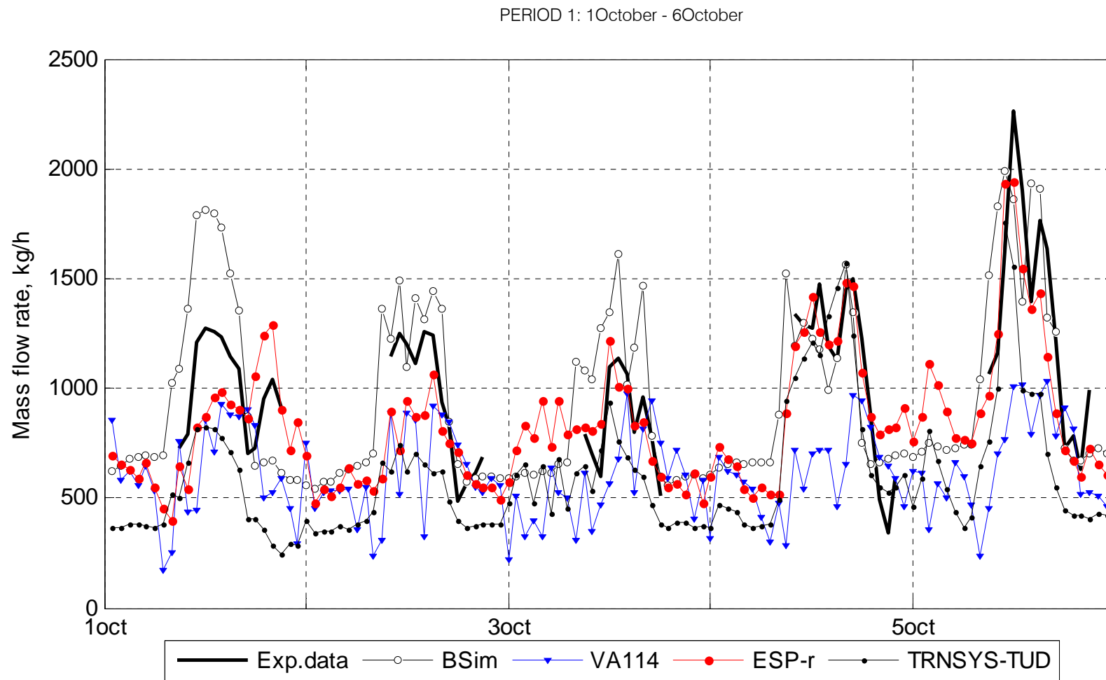
Figure 69. Hour averaged mass flow rate in the zone 1, measured with the velocity profile method. Velocity profile at h=1.91\text{m} (PERIOD 1: 1 October – 6 October).
