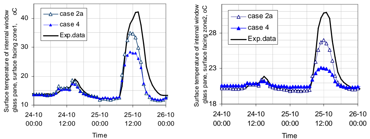
Figure 34. DSF100_e case with VA114 results for sensitivity cases 2a and 4.
