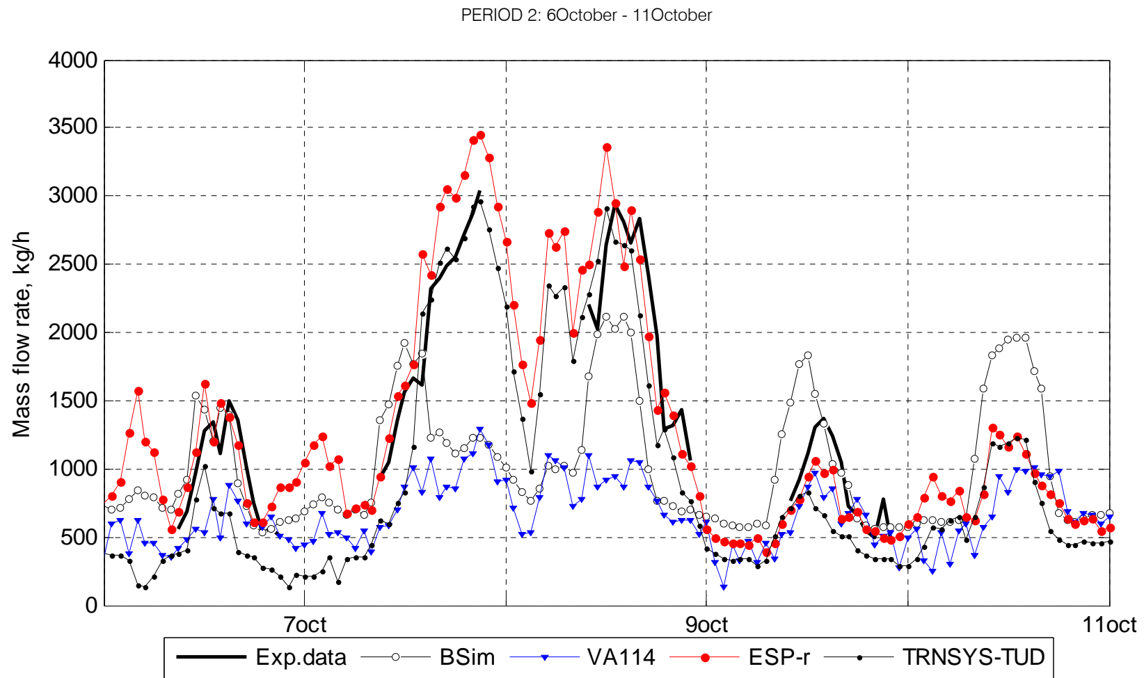
Figure 70. Hour averaged mass flow rate in the zone 1, measured with the velocity profile method. Velocity profile at h=1.91\text{m} (PERIOD 2: 6 October – 11 October).
