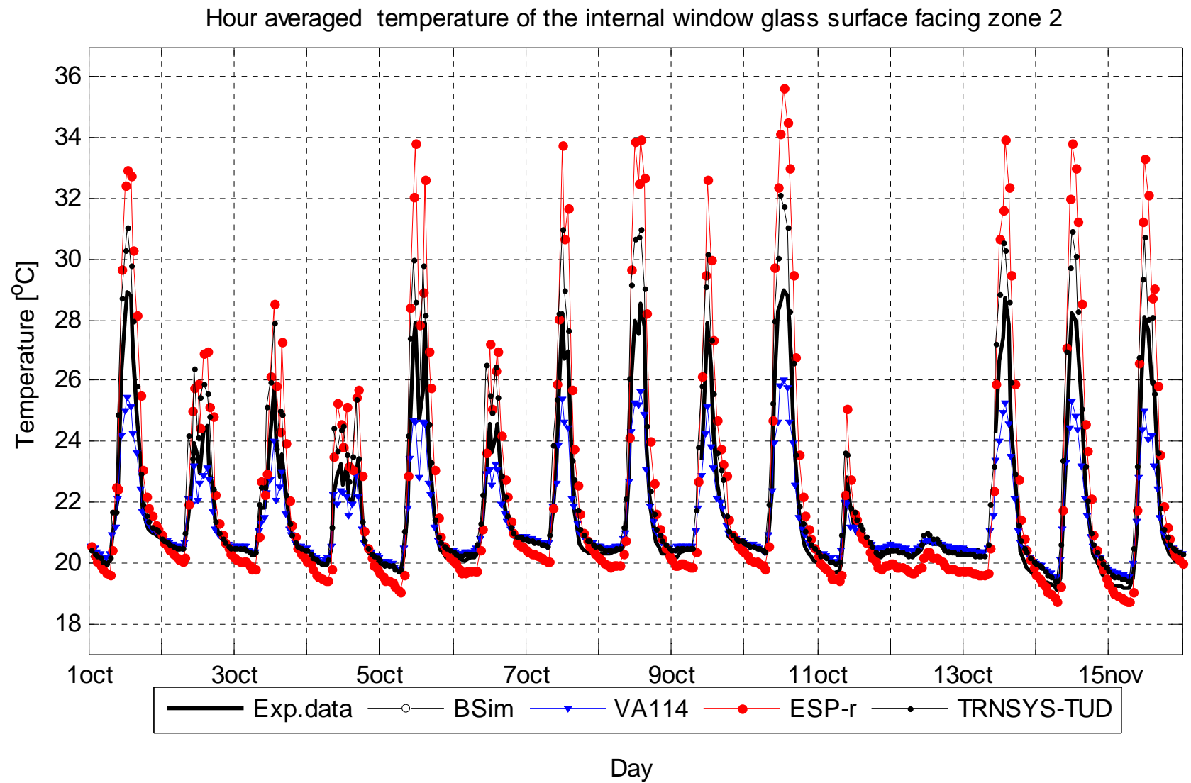
Figure 60. Temperature of the internal window glass surface facing zone 2. Test case DSF200_e.
