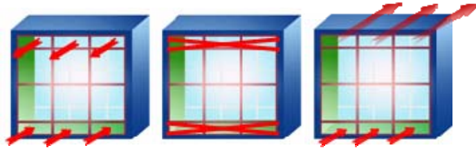
Figure 27. Operational modes of the DSF. External air curtain (left). Transparent insulation (centre). Preheating mode (right).
