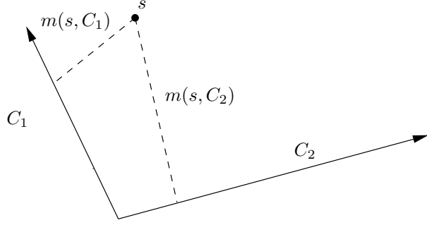
Fig. 4. Illustration of the decision rule of the discriminator. s is the defect in question. C_1 and C_2 are the centre of two groups. m(s, C_1) and m(s, C_2) are the measures of the distances between the defect in question and the respective group centres. Since s is closest to C_1 , this means that m(s, C_1) < m(s, C_2) . The decision is that the defect in this example is a member of group 1, since it is closest to centre of group 1.
