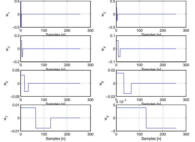
Fig. 3. The 8 generalised Haar basis vectors.
