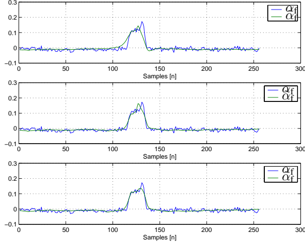
Fig. 2. Illustration of the Karhunen-Loève approximation of \alpha_f which contain a typical scratch. The first approximation is based on the one most approximating coefficient, the second approximation is based on the five most most approximating coefficients, and the third approximation on the seven most approximating coefficient.
