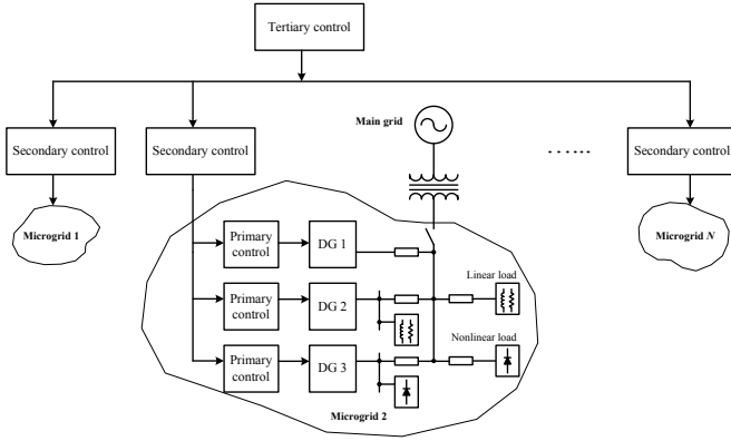
Fig. 1. The general structure for the hierarchical control of microgrids.
