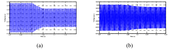
Fig. 13. The magnitude changes of the fifth and seventh harmonic voltages of the common load bus in the unsymmetrical case. (a) The fifth harmonic voltage. (b) The seventh harmonic voltage.
