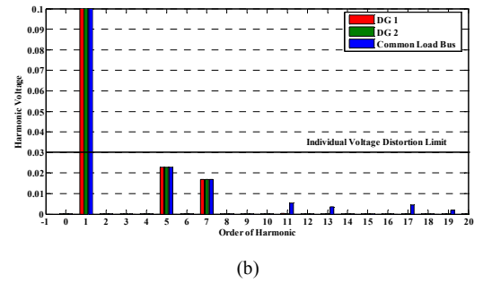
Fig. 14. The harmonic voltage spectrums in the unsymmetrical case. (a) Before applying the proposed method. (b) After applying the proposed method.
