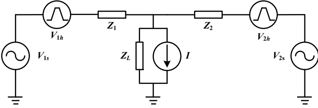
Fig. 5. Equivalent circuit of an islanded microgrid.
