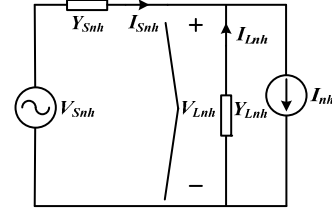
Fig. 7. Simplified equivalent circuit of the islanded microgrid.
