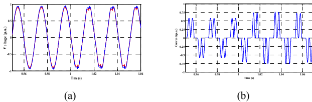
Fig. 12. The simulation waveforms of the unsymmetrical case when the proposed method is applying at the instant of 1 s. (a) Output voltages of DG units. (b) The harmonic current of three-phase diode rectifier.
