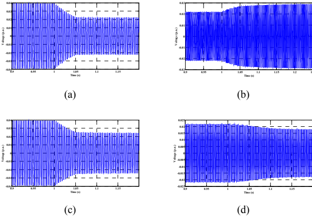
Fig. 11. The magnitude changes of the fifth and seventh harmonic voltages of the common load bus in the symmetrical case. (a) The fifth harmonic voltage when only the fifth harmonic voltage is of concern. (b) The seventh harmonic voltage when only the fifth harmonic voltage is of concern. (c) The fifth harmonic voltage when both the fifth and seventh are of concern. (d) The seventh harmonic voltage when both the fifth and seventh are of concern.
