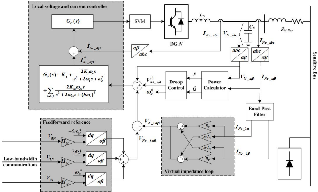
Fig. 3. The primary control system for DG unit N .
