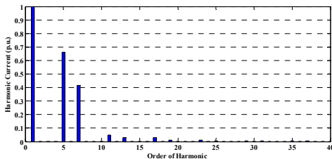
Fig. 8. The harmonic current spectrum for the three-phase diode rectifier.
