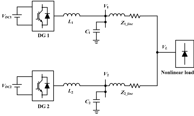
Fig. 4. A simplified one-line diagram of an islanded microgrid.
