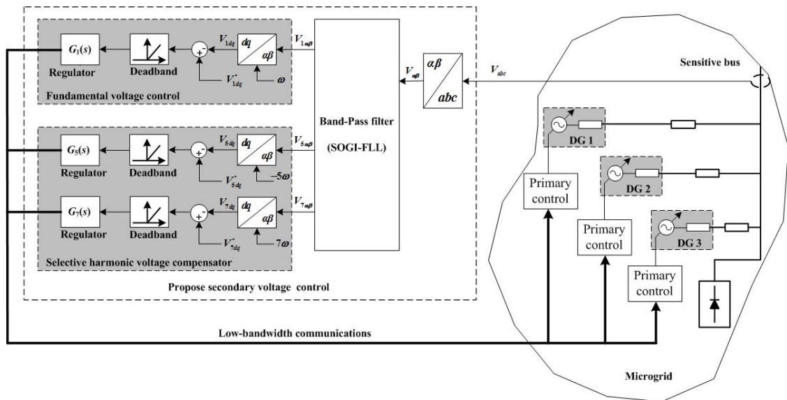
Fig. 2. The proposed secondary voltage control approach for harmonics suppression in an islanded microgrid.
