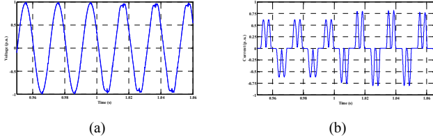
Fig. 10. The simulation waveforms for the symmetrical case when the proposed method is applying at the instant of 1 s. (a) Output voltages of DG units. (b) The harmonic current of three-phase diode rectifier
