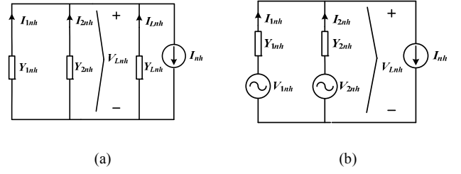
Fig. 6. The simplified equivalent circuits of the microgrid at the n th-order harmonic frequency. (a) Before applying the proposed method. (b) After applying the proposed method.
