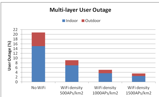
Fig. 3. Indoor/Outdoor Outage vs. Wi-Fi Density/ km 2
